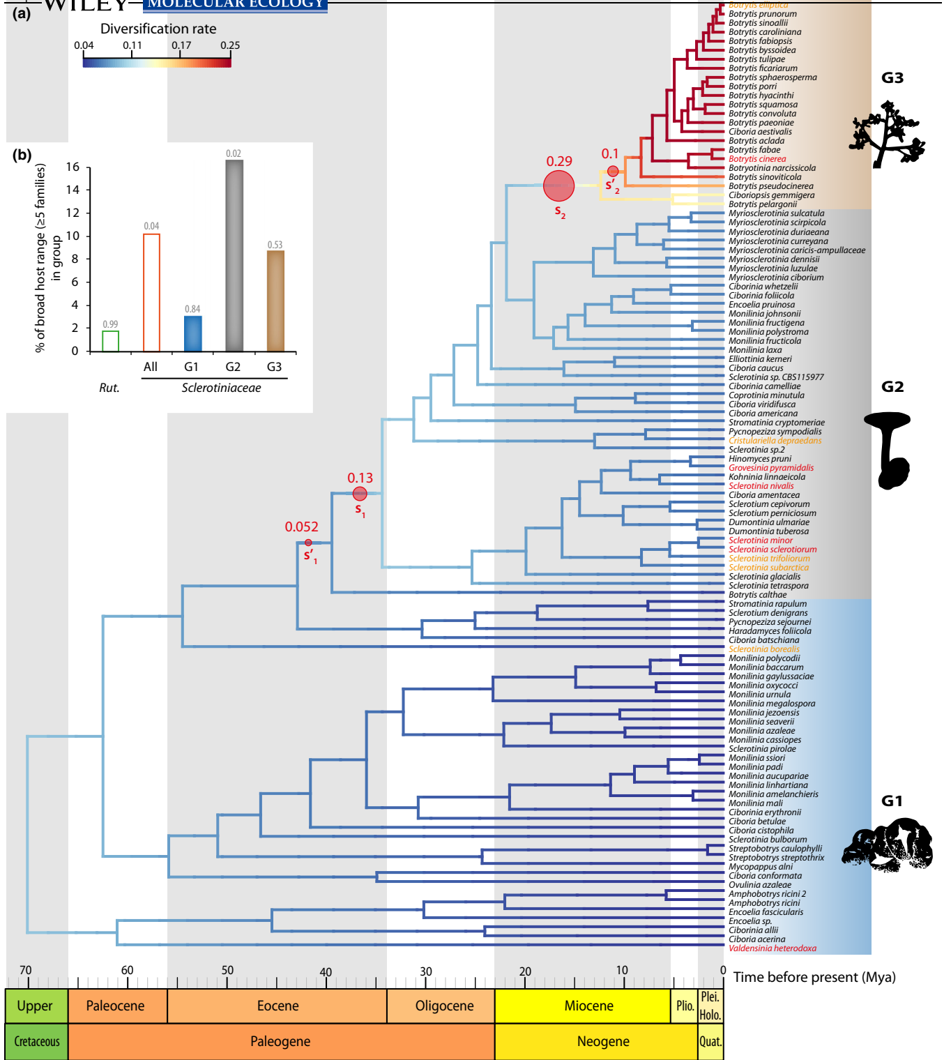
FIGURE 2 Two major diversification rate shifts in the evolution of the Sclerotiniaceae. (a) Dated ITS-based species tree for the Sclerotiniaceae with diversification rate estimates. The divergence times correspond to the mean posterior estimate of their age in millions of years calculated with BEAST. Mean age is shown for selected nodes with bars showing 95% confidence interval of the highest posterior density (HPD). Branches of the tree are colour-coded according to diversification rates determined with BAMM. Major rate shifts identified in BAMM are shown as red circles, noted s_1 , s'_1 , s_2 and s'_2 and labelled with the posterior distribution in the 95% credible set of macro-evolutionary shift configurations. Species names are shown in black if host range includes less than five plant families, in yellow for five to nine plant families and in red for 10 or more plant families. Diversification rate shifts define three macro-evolutionary regimes noted G1, G2 and G3 and boxed in blue, grey and brown, respectively. (b) Distribution of broad host range (five or more host families) parasites in Rutstroemiaceae, Sclerotiniaceae and under each macro-evolutionary regime of the Sclerotiniaceae. p-Values calculated by random permutations of host ranges along the tree are indicated above bars. Holo., Holocene; Mya, Million years ago; Plei., Pleistocene; Plio., Pliocene; Quat. Quaternary; Rut., Rutstroemiaceae
