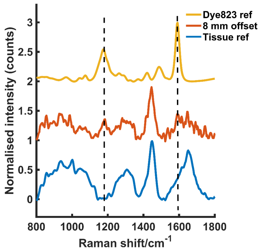
Figure 3 - The tracking of dye 823 nanotag solution through 25 mm of tissue. The tissue and dye823 reference spectra are shown at the bottom and top respectively. The middle spectrum represents the Raman signal collected at an 8 mm offset through 25 mm of tissue. The peak at 1178\text{ cm}^{-1} is easily detectable by eye and the peak at 1592\text{ cm}^{-1} is also detectable, albeit to a lesser extent. All measurements were carried out using a 2 s integration time, 5 accumulations, 830 nm laser excitation wavelength.
