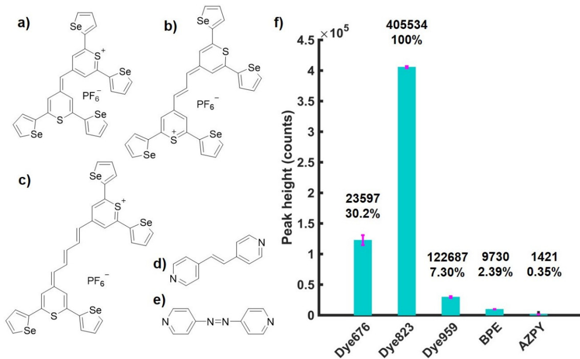
Figure 1- (a – e) Chemical structure of dye676, dye823, dye959, BPE and AZPY respectively. (f) Bar chart showing average peak intensities of dye676, dye823, dye959, BPE and AZPY at 1598, 1592, 1572, 1201 and 1162 \text{cm}^{-1} respectively, as well as the relative percentage peak intensity, through 5 mm of tissue. Nanotag solutions were held in a cuvette and the cuvette was placed behind tissue samples. Spectra were collected using a handheld SORS instrument with 830 nm laser excitation at an 8 mm offset. Peak intensities were obtained by scanning 3 replicate samples, 5 times (2 second integration, 5 accumulations). The average peak intensity for each of the 5 dyes is shown and error bars represent \pm one standard deviation.
