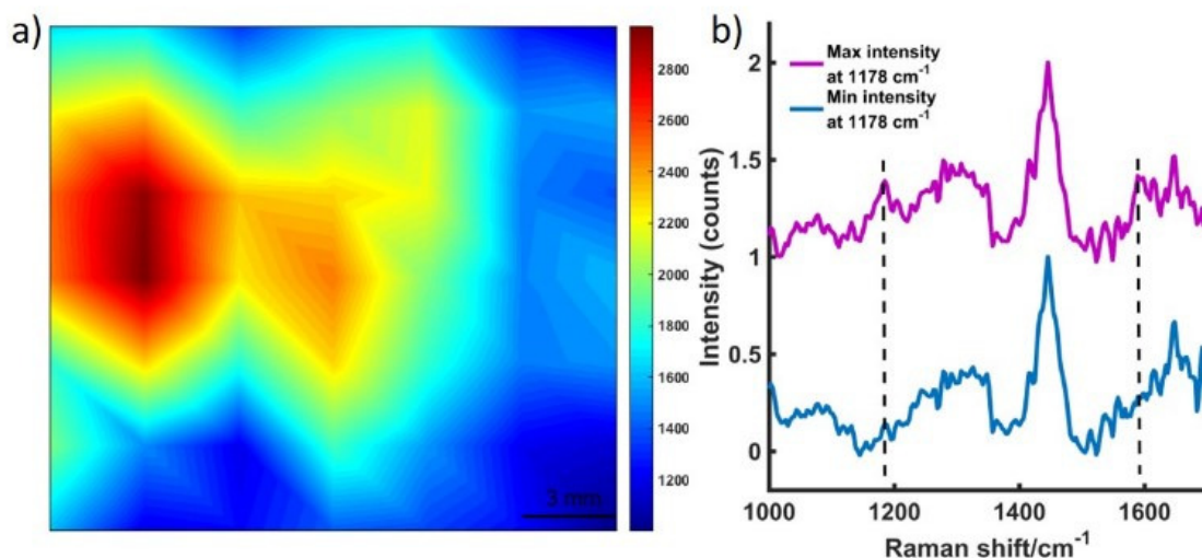
Figure 2 (a) A false colour xy-2D heat SESORRS map of MTS containing dye823 through 15 mm of tissue. The map was constructed using the peak intensity at 1178 \text{cm}^{-1} . Measurements were carried out using an xy translational stage in step sizes of 3 mm to create an image of 7 \times 7 pixels. Spectra were truncated, baselined and smoothed prior to processing. A combination surface/contour false colour was used to generate a 2D heat map and show the tracking of the MTS through 15 mm of tissue. Clear discrimination is seen between spectra collected at the point of maximum intensity where the nanotags were spotted and that collected where the nanotags were not present. (b) The corresponding maximum and minimum collected 8 mm offset spectra. All measurements were carried out using a 2 s integration time, 5 accumulations, 830 nm laser excitation wavelength.
