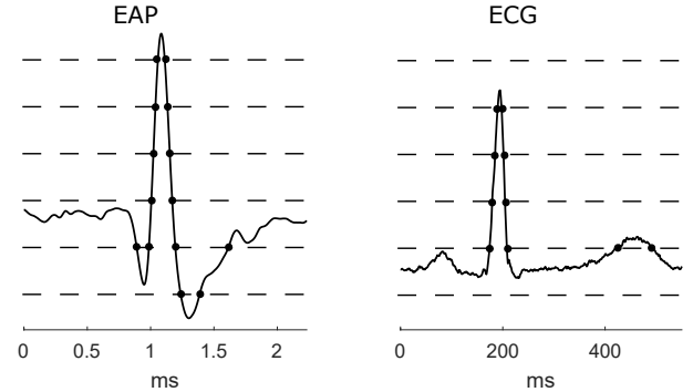
Fig. 1. Example of using CT sampling for EAP and ECG representation (showing a 3-bit converter for simplicity).
