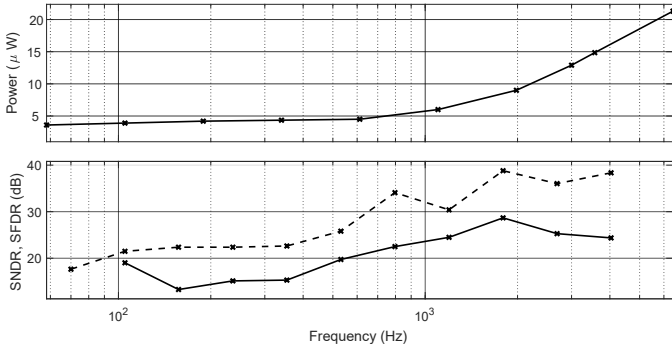
Fig. 13. Power consumption, SFDR (dashed) and SNDR (solid) obtained after converting a sinusoidal input.
