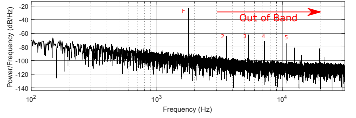
Fig. 14. Output spectrum of a reconstructed 200 \text{ mV} , 1794 \text{ Hz} sine wave passing through 256 quantisation levels (8 bits) showing an SNDR of 28.65 \text{ dB} (ENOB of 4.47 bits) and SFDR of 38.8 \text{ dB} .
