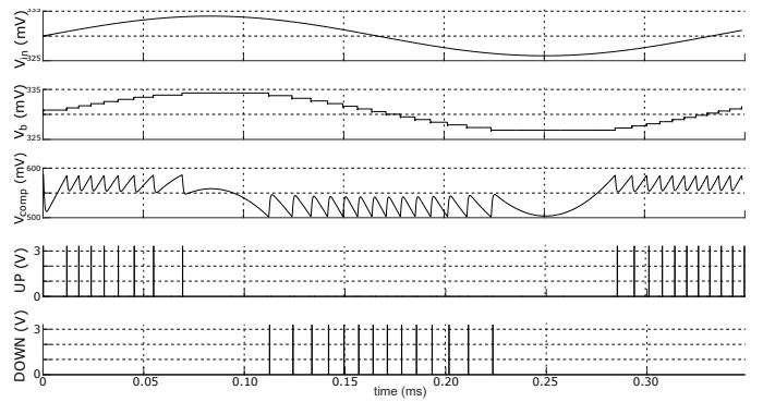
Fig. 8. Sample waveforms of V_{in} , V_b and V_{comp} alongside output signals indicating operation of the presented CT-ADC.
