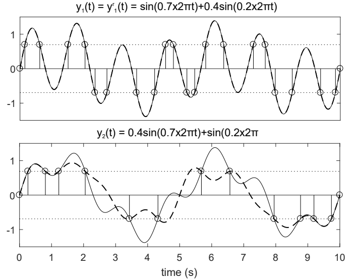
Fig. 5. Demonstration of aliasing occurring in CT-sampled signal. Solid line - original signal, Dotted line - quantisation levels, Dashed line - reconstructed signal using sinc interpolation method for non-uniformly sampled signals [39]. Top: Signal y_1(t) = y_1^r(t) reconstructed without aliasing, Bottom: Signal y_2(t) subject to aliasing resulting in y_2^r(t) \neq y_2(y) .
