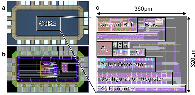
Fig. 12. a) A microphotograph of the fabricated circuit, b) Layout of the circuit exported from Cadence, c) A close-up of annotated layout exported from Cadence. 1 - Input Comparator, 2 - Unity Gain Buffer, 3 - Threshold Crossing Detector, 4 - Charge Injection Circuits, 5 - Debugging Voltage Followers. Adapted from [27] and modified.
