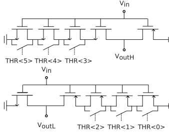
Fig. 9. Configurable threshold crossing detector circuit (Up - top, Down-bottom). All devices are minimum size ( W/L = 0.4/0.35 ). Adapted from [27].
