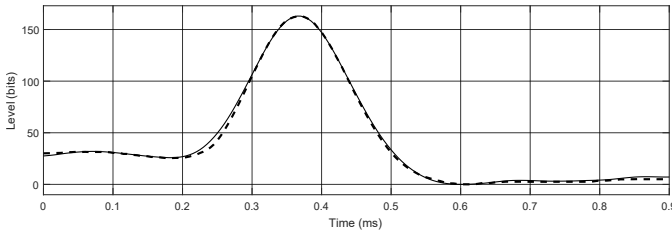
Fig. 18. An example of a reconstructed neural spike (dashed) and the original signal (solid) passing through 164 quantisation levels.
