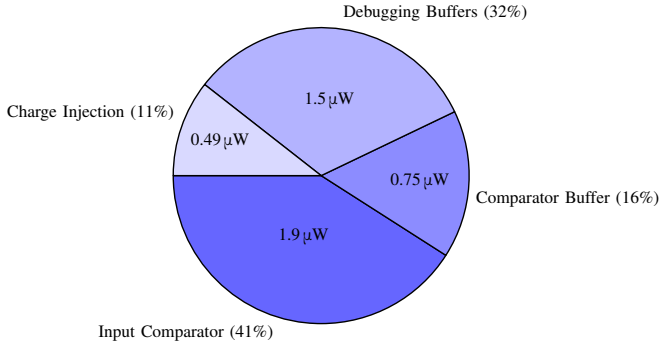
Fig. 17. Power consumption of each block in the system.
