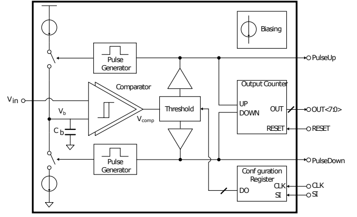
Fig. 7. High-level block diagram of the proposed CT-ADC implementation. Adapted from [27] and modified.
