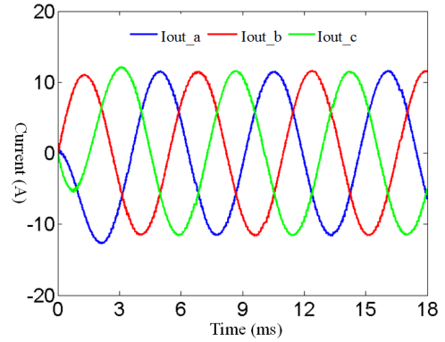
(a) Output current under normal operation condition
