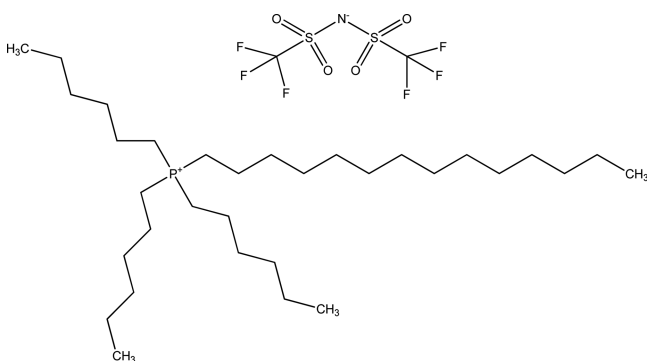
Figure 4. Trihexyl(tetradecyl)phosphonium bis[(trifluoromethyl)sulfonyl]imide ( [\text{P}_{66614}][\text{Tf}_2\text{N}] ).
