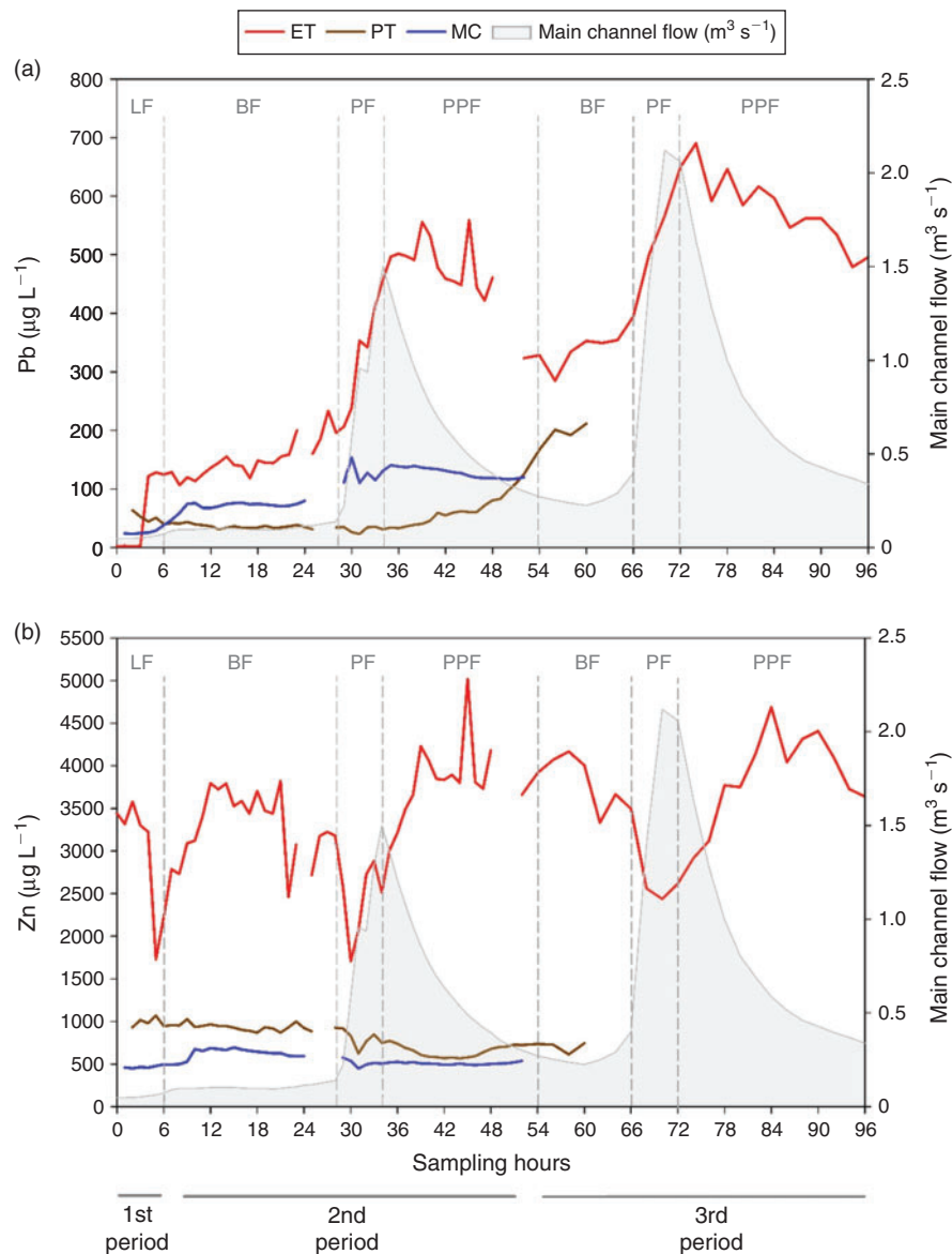
Fig. 1. Trends of metal concentrations ( \mu\text{g L}^{-1} ) at different sites during three rainfall periods. Panel (a) shows trends of Pb concentrations, and Zn concentrations are indicated in panel (b). The secondary y axis shows flow data collected at the gauging station in the main channel. Solid lines represent sampling sites and shaded area flow data. Perpendicular dotted lines indicate the flow stages at different rainfall periods (ET, ephemeral tributary; PT, perennial tributary; MC, main channel).
