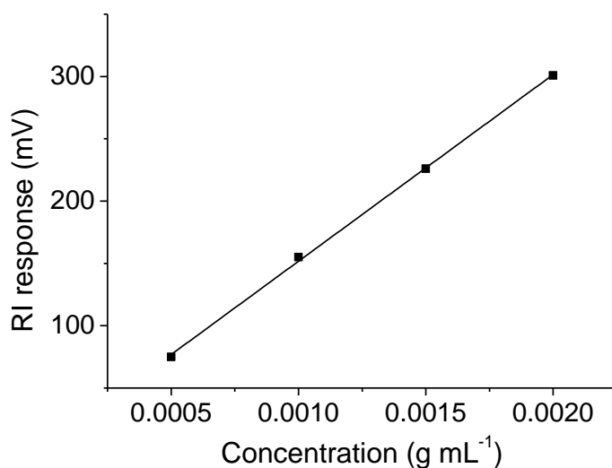
Figure S2: Plot of concentration vs RI response for 2 in salt solution. The dn/dc was calculated as 0.130 mL g -1 using the slope of the linear fit.
