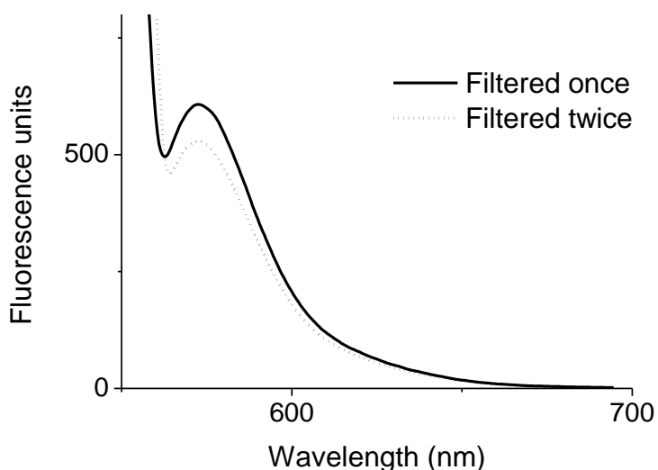
Figure S10: Fluorescence spectra showing the effect of filtering the micelle solution of 2' multiple times has on the fluorescence response ( \lambda_{\text{ex}} = 500 nm) following incubation with Nile Red.
