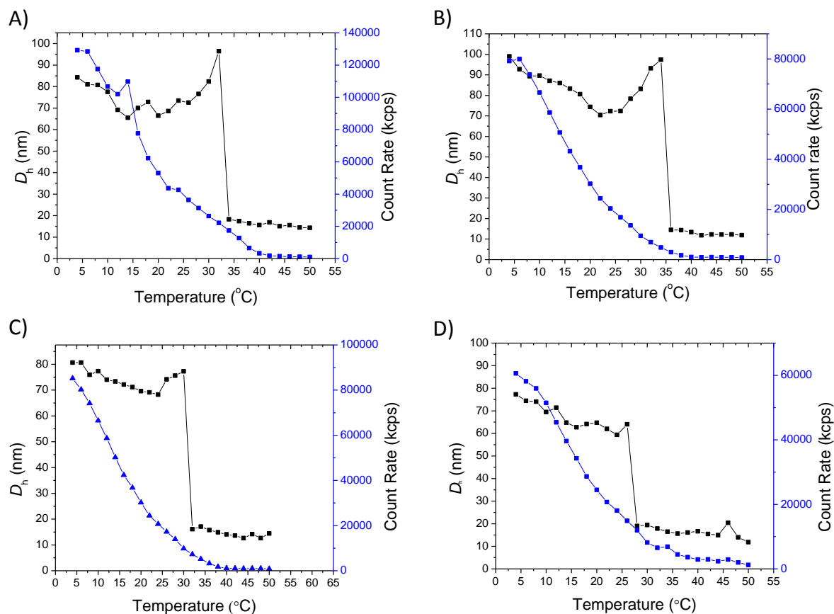
Figure S7: Plots of count rate ( \blacktriangle ) and size ( \blacksquare , D_h ) with increasing temperature for A) 2' in water, B) 3' in water, C) 4' in water, D) 5' in water.
