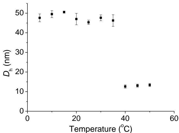
Figure S8: DLS analysis with temperature of 2' at 5\text{ mg mL}^{-1} . Error bars are one standard deviation calculated from at least three measurements at each temperature.
