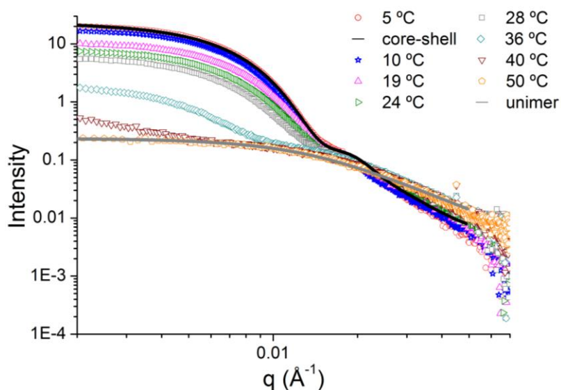
Figure S6: SAXS profiles for 2' at varying temperatures between 5 °C and 50 °C in water with a core-shell fit shown as a solid line.
