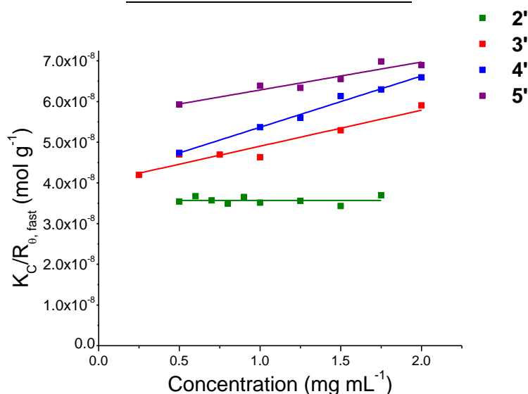
Figure S5: Plot of Kc/R_{\theta, fast} vs concentration for self-assembled solutions 2' , 3' , 4' and 5' in water at 20°C. The M_w was calculated using the intercept of the linear fit to the SLS data.
