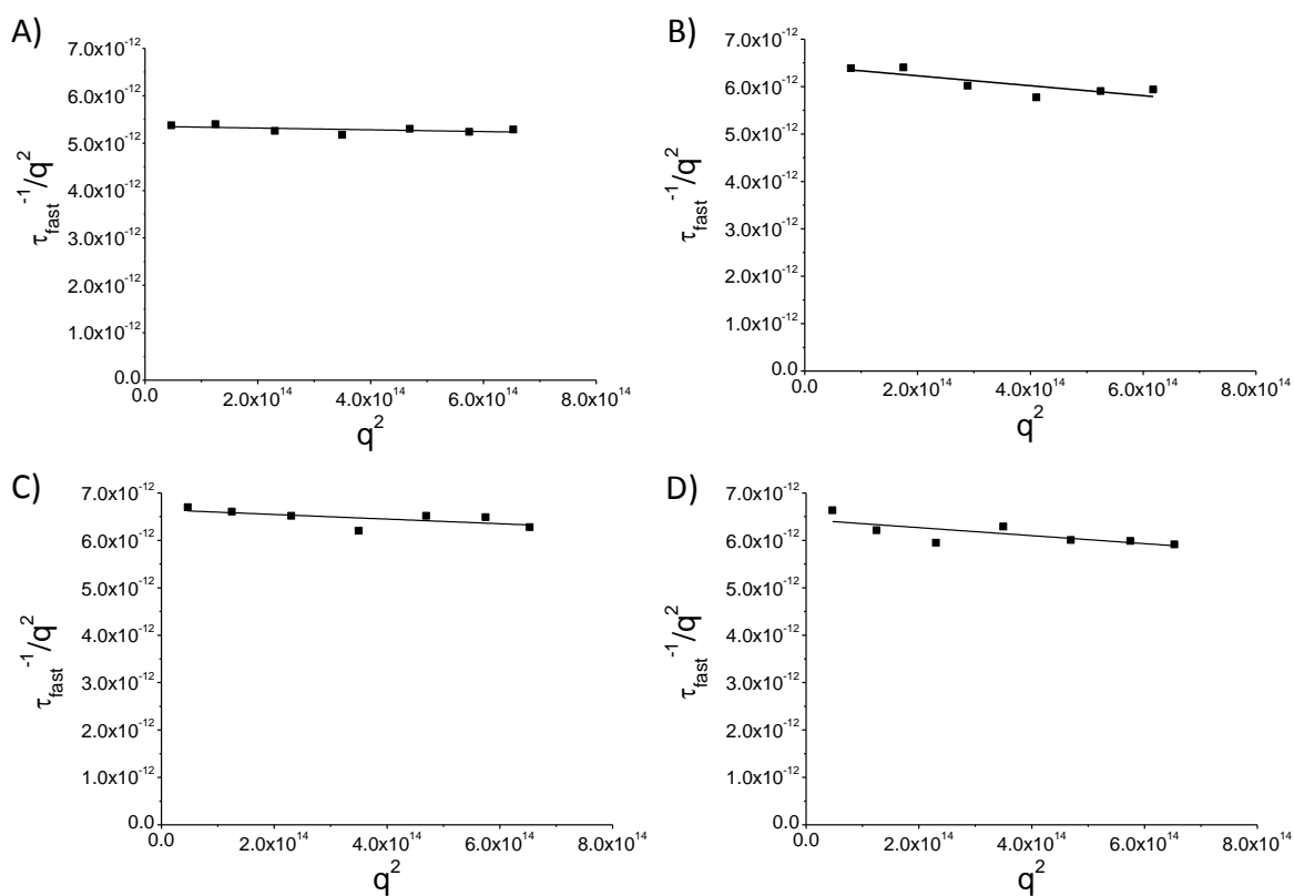
Figure S4: Plots of \tau_{\text{fast}}^{-1}/q^2 vs q^2 for A) 2' at 1 mg mL -1 , B) 3' at 1 mg mL -1 , C) 4' at 1 mg mL -1 , D) 5' at 1 mg mL -1 , showing there to be no significant angular dependence of the scattering of the self-assembled solutions.
