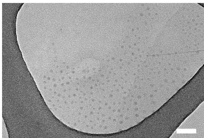
Figure S14: Dry-state TEM image of 5', at 0.1mg mL -1 , imaged on a graphene oxide support, scale bar 100nm showing the dissociation of the micelles on the graphene oxide support.
