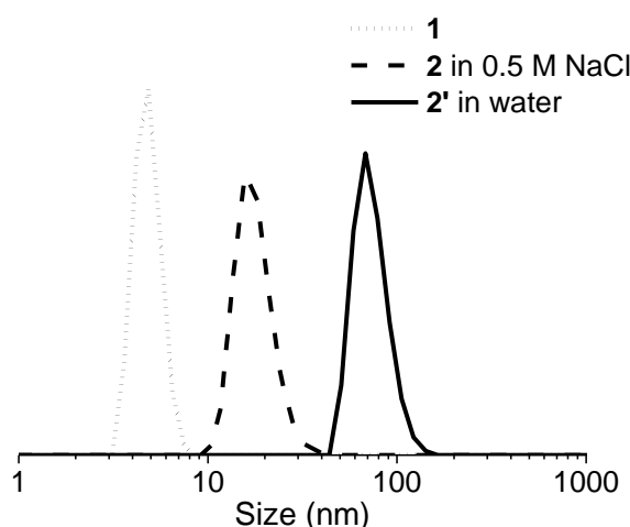
Figure S1: Number average DLS traces of POEGMA homopolymer 1 ( D_h = 5 \pm 1 \text{ nm} ), diblock copolymer 2 in 0.5 \text{ M NaCl} solution ( D_h = 18 \pm 1 \text{ nm} ), and diblock copolymer 2' in pure water ( D_h = 74 \pm 2 \text{ nm} ), determined at 25 \text{ }^\circ\text{C} , all at 1 \text{ mg mL}^{-1} .
