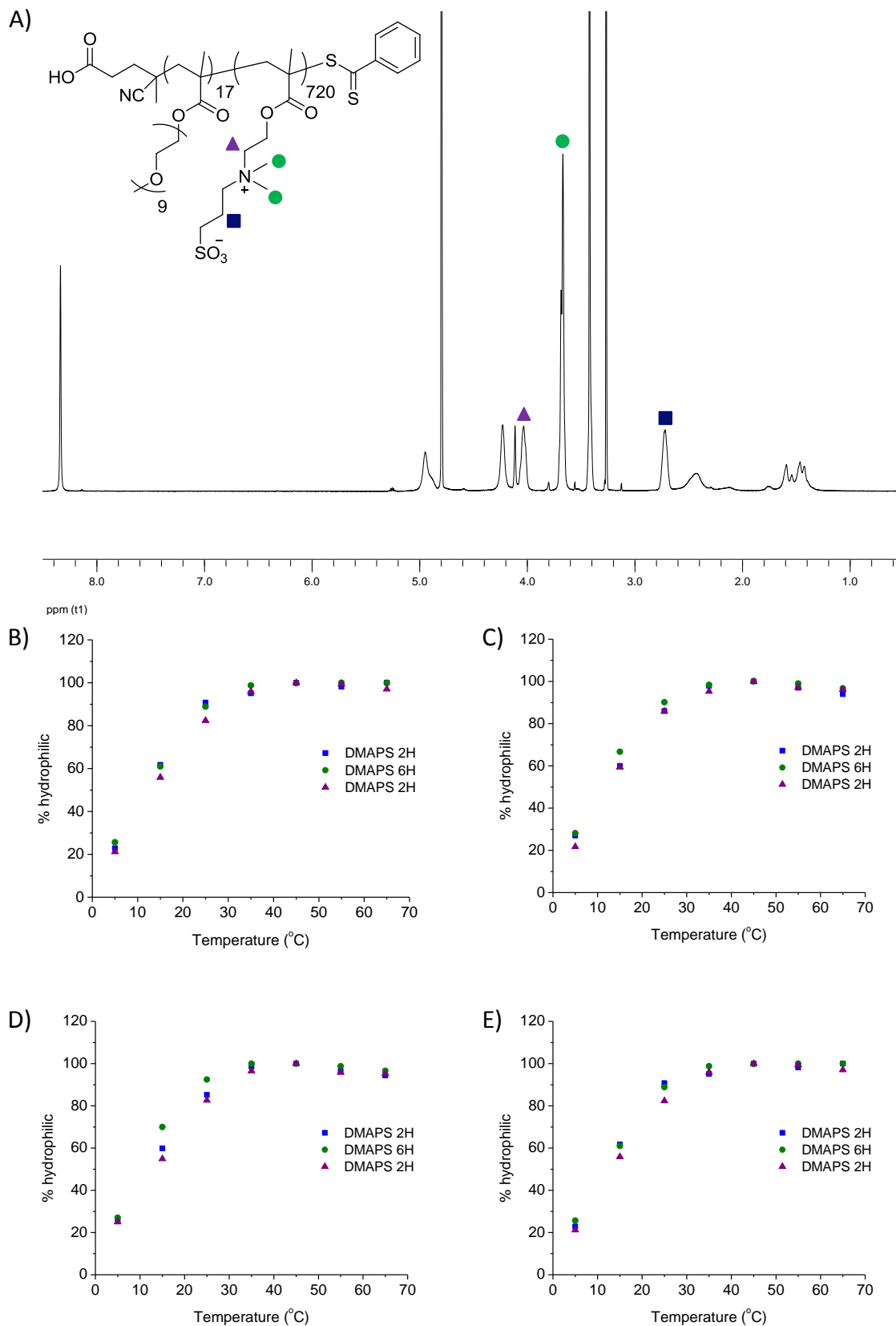
Figure S9: A) ^1\text{H} NMR spectrum showing the three DMAPS peaks used for calculating remaining hydrophilicity in 2' , and B) – E) plots showing how the % relative hydrophilicity of the DMAPS segment of diblock copolymers 2' – 5' , respectively, change with increasing temperature.
