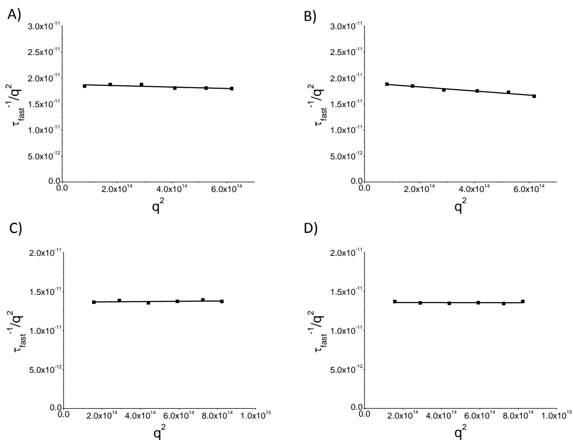
Figure S3: Plots of \tau_{\text{fast}}^{-1}/q^2 vs q^2 for A) 2 at 1 mg mL -1 in 0.5 M NaCl, B) 3 at 1 mg mL -1 in 0.5 M NaCl, C) 4 at 1 mg mL -1 in 0.5 M NaCl, D) 5 at 1 mg mL -1 in 0.5 M NaCl, showing there to be no significant angular dependence of the scattering of the dissolved polymer chains.
