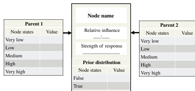
Figure 2. Example of tool for translating expert knowledge into a Conditional Probability Table (CPT) for use in a Bayesian Network.
