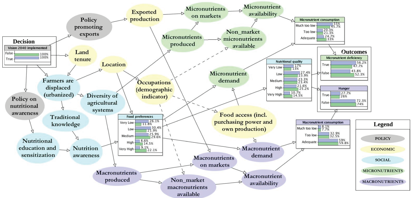
Figure 3. Bayesian Network (BN) for impact of Vision 2040 on household nutrition in Uganda. Probabilities are shown (boxes) for outcome variables and variables with the highest value of information. Green bars show the probabilities for the node states for the scenario that the Vision 2040 decision is not implemented ("Vision 2040 false"), and blue bars show probabilities for the scenario that the Vision 2040 decision is implemented ("Vision 2040 true"). Data set and AgenaRisk model available online (Luedeling & Whitney, 2017).
