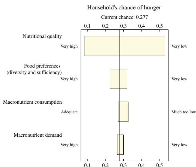
Figure 4. Sensitivity analysis of a Bayesian Network for probability of household hunger within 10 years of the implementation of Vision 2040.
