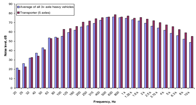
(b) Car transporter (5 axles) unladen
