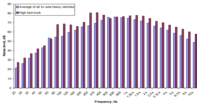
(a) High load bed truck (3 axles)
