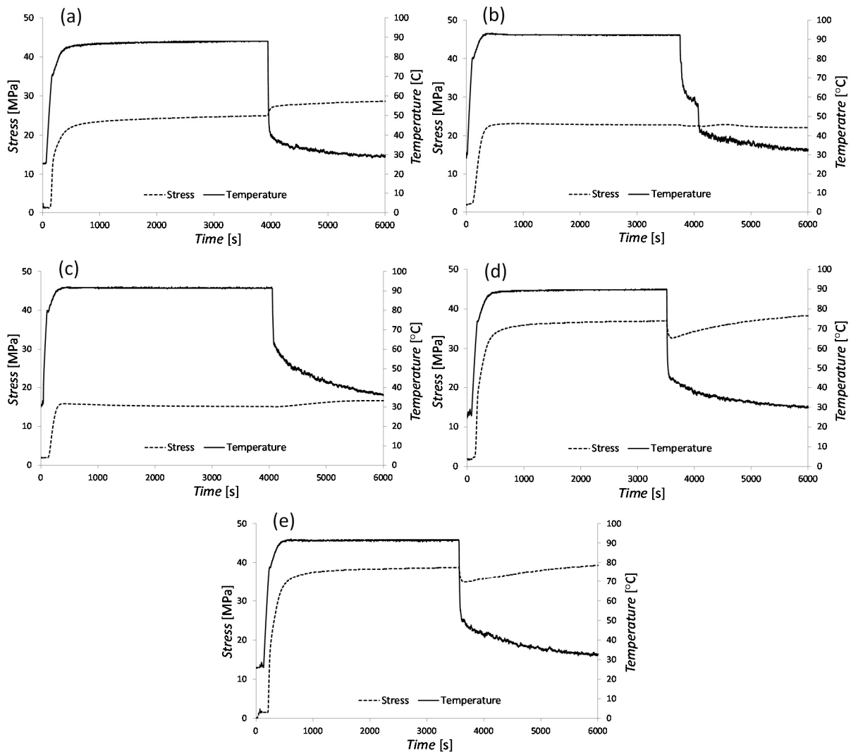
FIGURE 4 Restrained shrinkage stress at 90°C for (a) Strips; (b) Tube; (c) Tube with filaments; (d) Solid filaments & (e) Filament tube. Typical results graphs shown for samples with repetitions.
