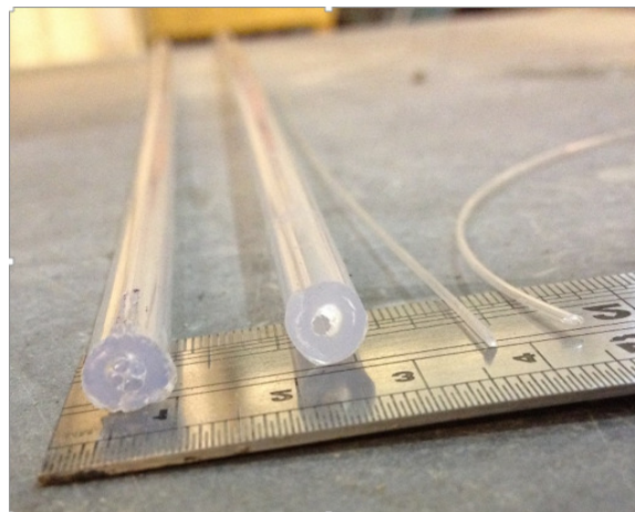
FIGURE 2 Manufactured PET samples, left to right: tube with filaments, tube, solid filament, filament tube
