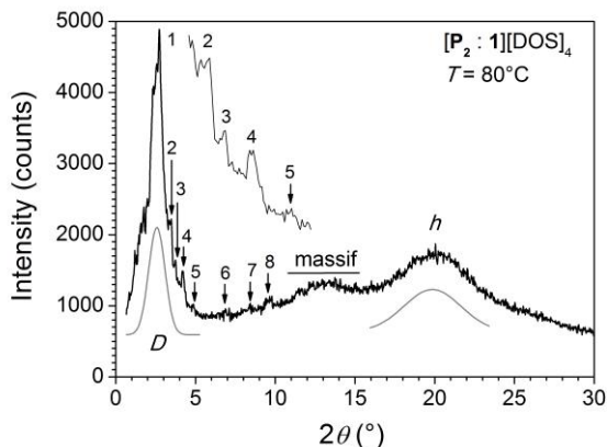
Figure 8. Representative SAXS patterns of [P_2\subset 1][DOS]_4
