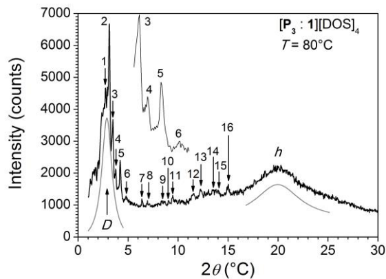
Figure 7. Representative SAXS patterns of [P_3\subset 1][DOS]_4
