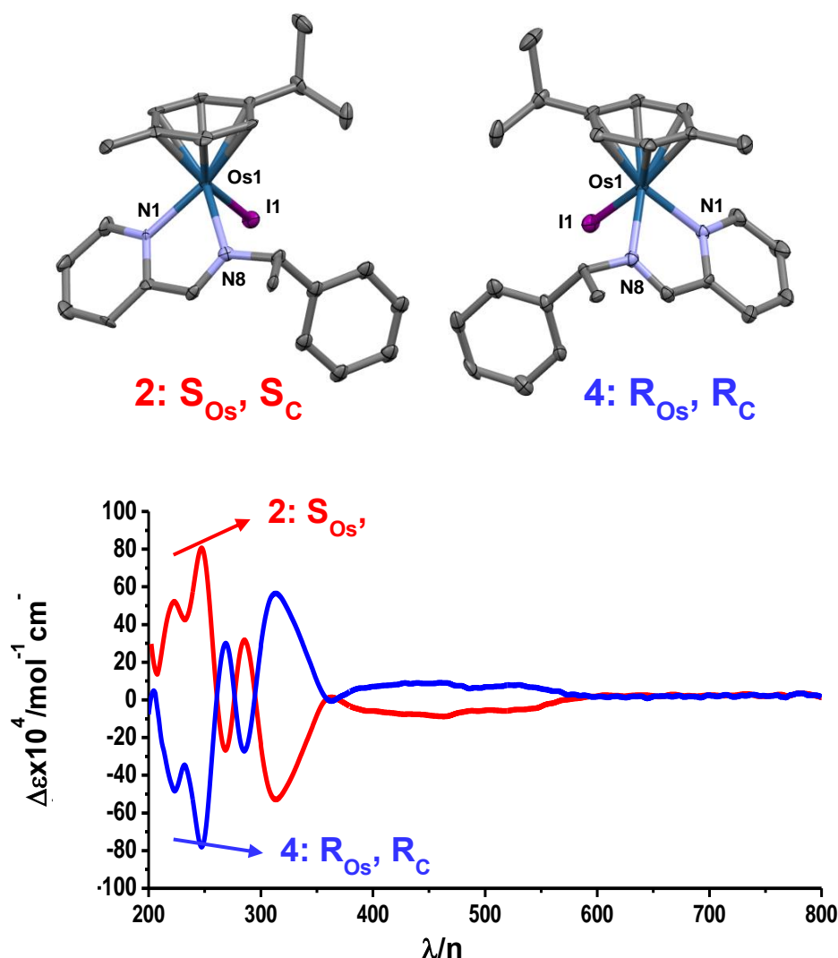
Figure 12. X-ray crystal structures of enantiomeric p -cymene Os II iminopyridine complexes and their CD spectra. Adapted from ref 100
