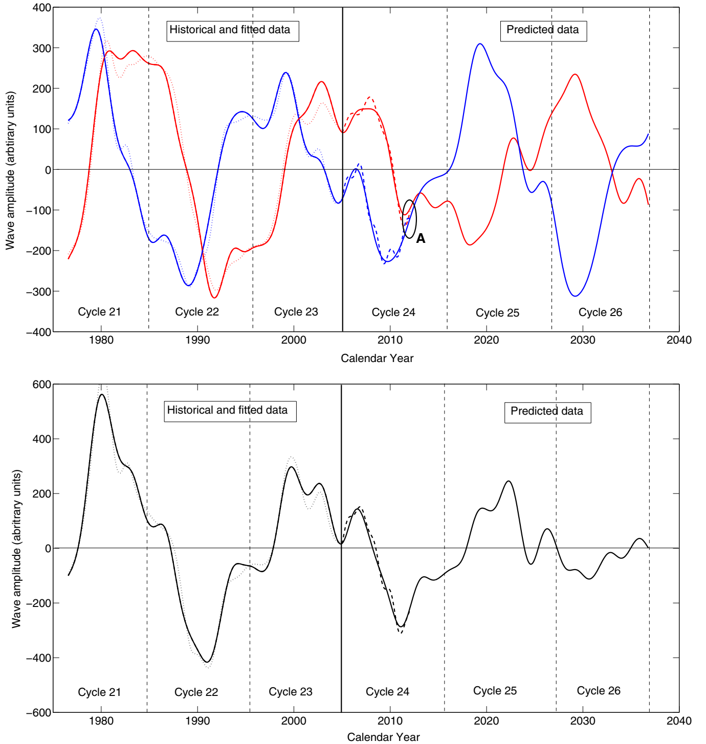
Figure 2. Top plot: the accuracy of the fit with distilled laws from Eureqa (solid curves) to the two principal components (PCs) of SBMF (dotted curves) from Figure 1 for cycles 21–23 and their further expansion to cycles 24–26. Bottom plot: the fit of the Eureqa -distilled law (the solid curve) to the summary component in cycles 21–23 (dotted curve) and its expansion to cycles 24–26. Dashed curves in both plots show the predicted principal components (top plot) and the summary curve (bottom plot) compared to the real PCs derived from the SBMF in the cycle 24 with an accuracy better than 98%. A letter “A” denotes summer 2014.
