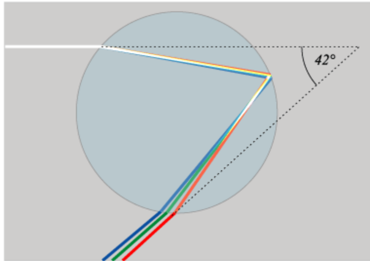
Figure 3: Double refraction and single reflection in a water drop, giving rise to a primary rainbow; \delta = 42^\circ
