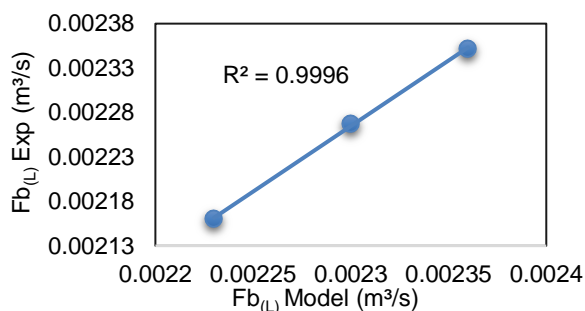
Figure 2: Linear fitting of experimental and model prediction of outlet feed flow rate
