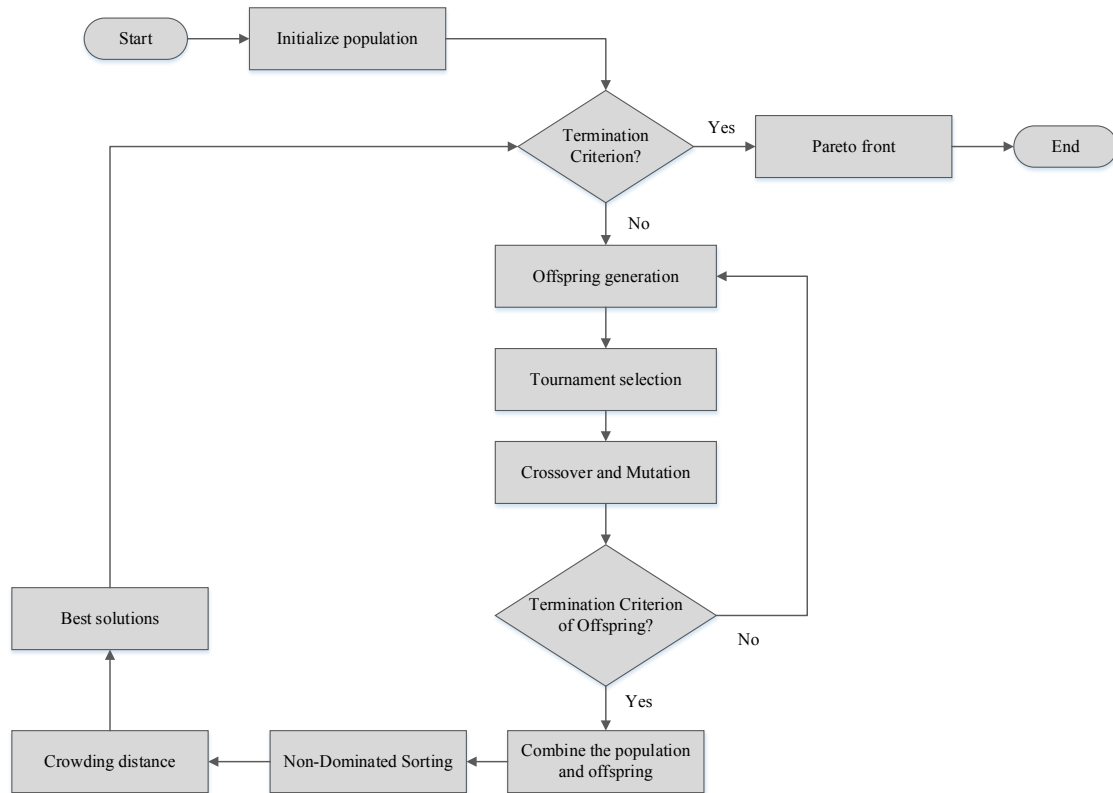
Fig. 7. Flowchart of NSGA-II
