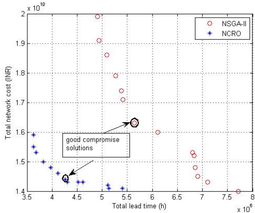
Fig. 10 (a). Obtained Pareto-fronts of the algorithms for problem instance 3
