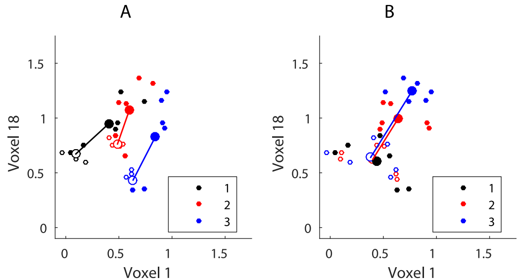
Fig 10. The transformation of response values for two voxels as a result of interference ( \beta = 0.5 ). Small circular markers depict response patterns, larger circular markers depict pattern means. Empty markers depict the original patterns and means, filled markers depict the data after simulating the interference process. Solid lines depict the movement of class means as a result of interference. (A) Item information. (B) Position information.
