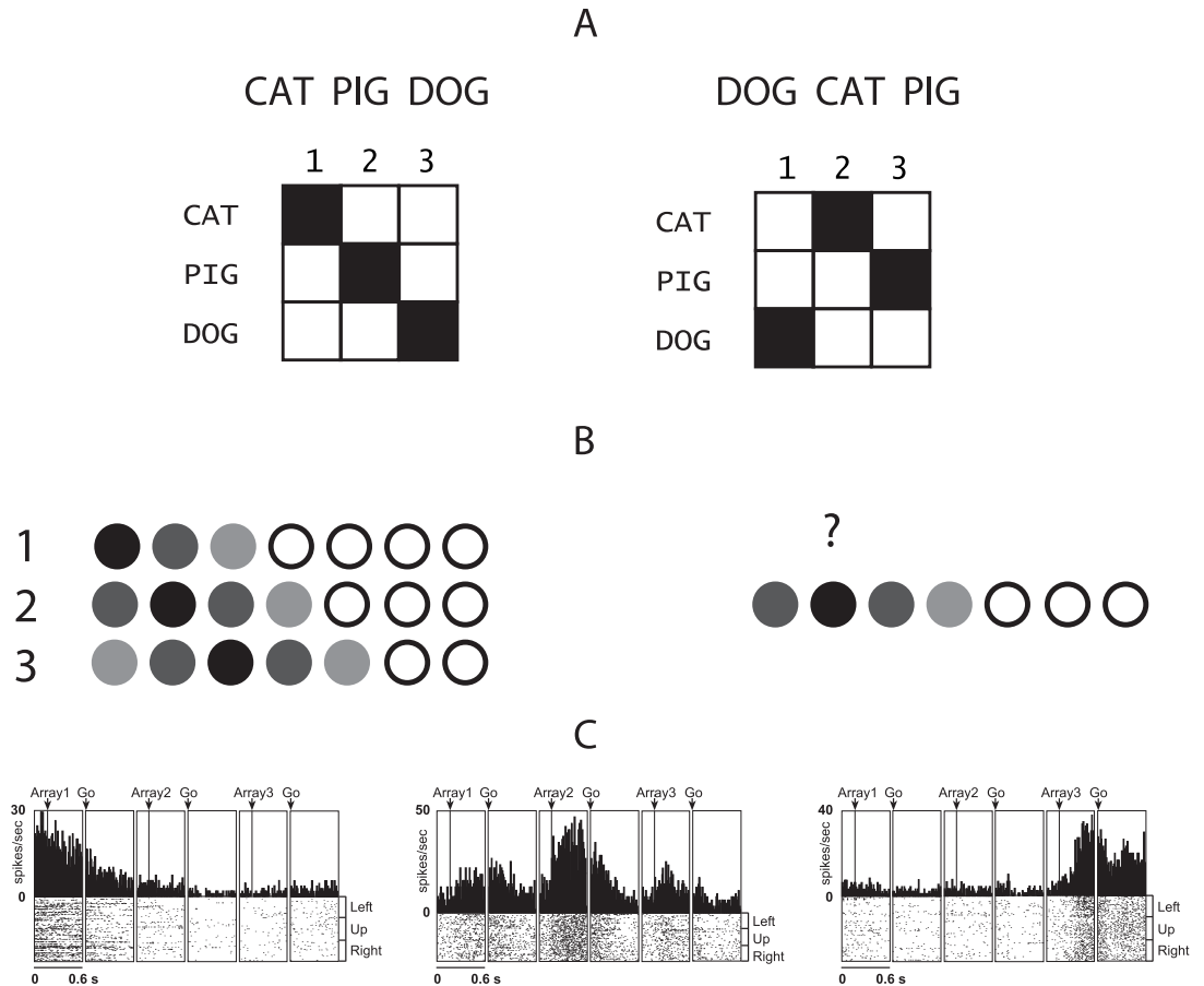
Fig 1. Sequence representation and temporal position. (A) Representation of two sequences as mappings between item codes and temporal position codes. (B) Left: representation of temporal position in a 7-item sequence. The variance around positional signal is coded in terms of the darkness of the circle. Right: the order position is retrieved by reinstating each positional code which then cues the associated item. (C) Examples of temporal position selective neurons from [7]. From left to right: pre-supplementary motor area neuron selective for 1st position, supplementary eye field neuron selective for 2nd position, and supplementary motor area neuron selective for the 3rd position in the serial object task.
