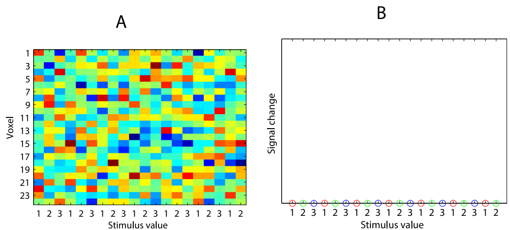
Fig 8. Simulation of sensory adaptation, z-scoring. (A) Voxels' responses with sensory adaptation, z-scored. (B) Average responses of voxels as column-wise means of the response matrix.
