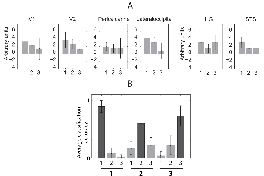
Fig 2. Sensory adaptation in the sensory cortex and decoding order position. (A) Uniform signal change over 3-item sequences in sensory brain areas averaged across participants. Data from visual regions V1, V2, pericalcarine, and lateraloccipital regions is from [33]. Data from auditory areas Heschl's gyrus (HG) and superior temporal sulcus (STS) is from [32]. (B) Distribution of average linear classification accuracy values of item position in V1 region across participant's from [33]. Bar charts display the average classification accuracy across participants by comparing the known positions (labels) to the predictions made by the classification algorithm. Bars show the proportion of predicted values for each position. Correct classifications are represented with a darker bar. Error bars show the standard error of the mean. The red line depicts the chance level classification accuracy 1/3.
