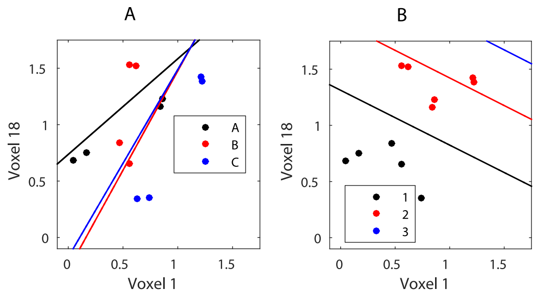
Fig 11. LDA between-class boundaries for two voxels, interference \beta = 0.5 . (A) Item information. (B) Position information.
