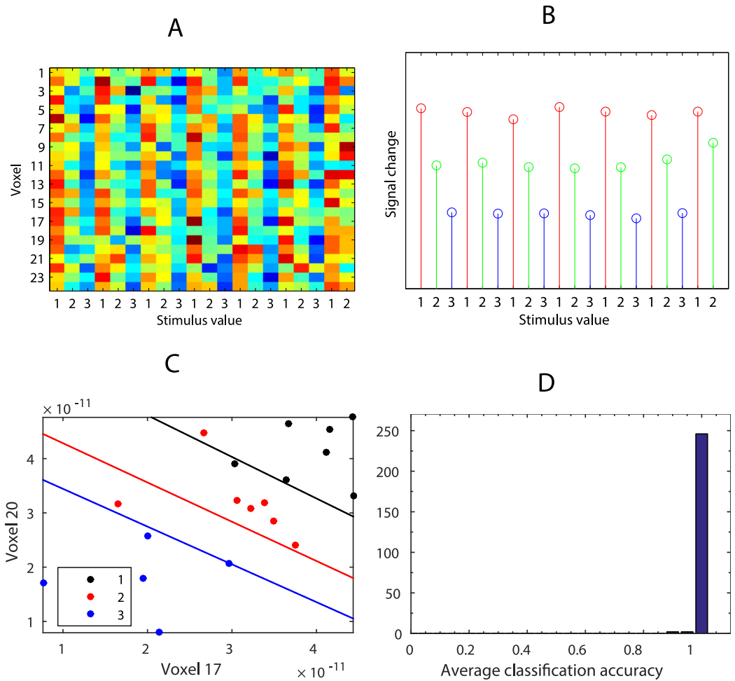
Fig 7. Simulation of sensory adaptation. (A) Voxels' responses with sensory adaptation. (B) Average responses of voxels as column-wise means of the response matrix. (C) LDA between-class boundaries based on the two most informative voxels. (D) Distribution of average LDA accuracy values (based on 250 simulations).
