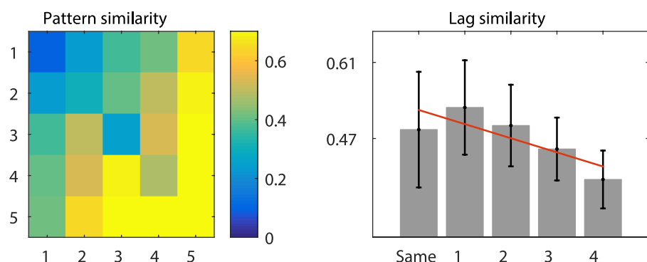
Fig 13. Positional pattern similarity decreases as a function of lag. Similarity matrix on the left shows average positional pattern similarity, as measured by Pearson's \rho , based on additive interference with \beta = 0.8 . Plot on the right visualises this similarity as a function of positional lag. The red line depicts a statistically significant negative slope over positional lag ( p < 0.05 ).
