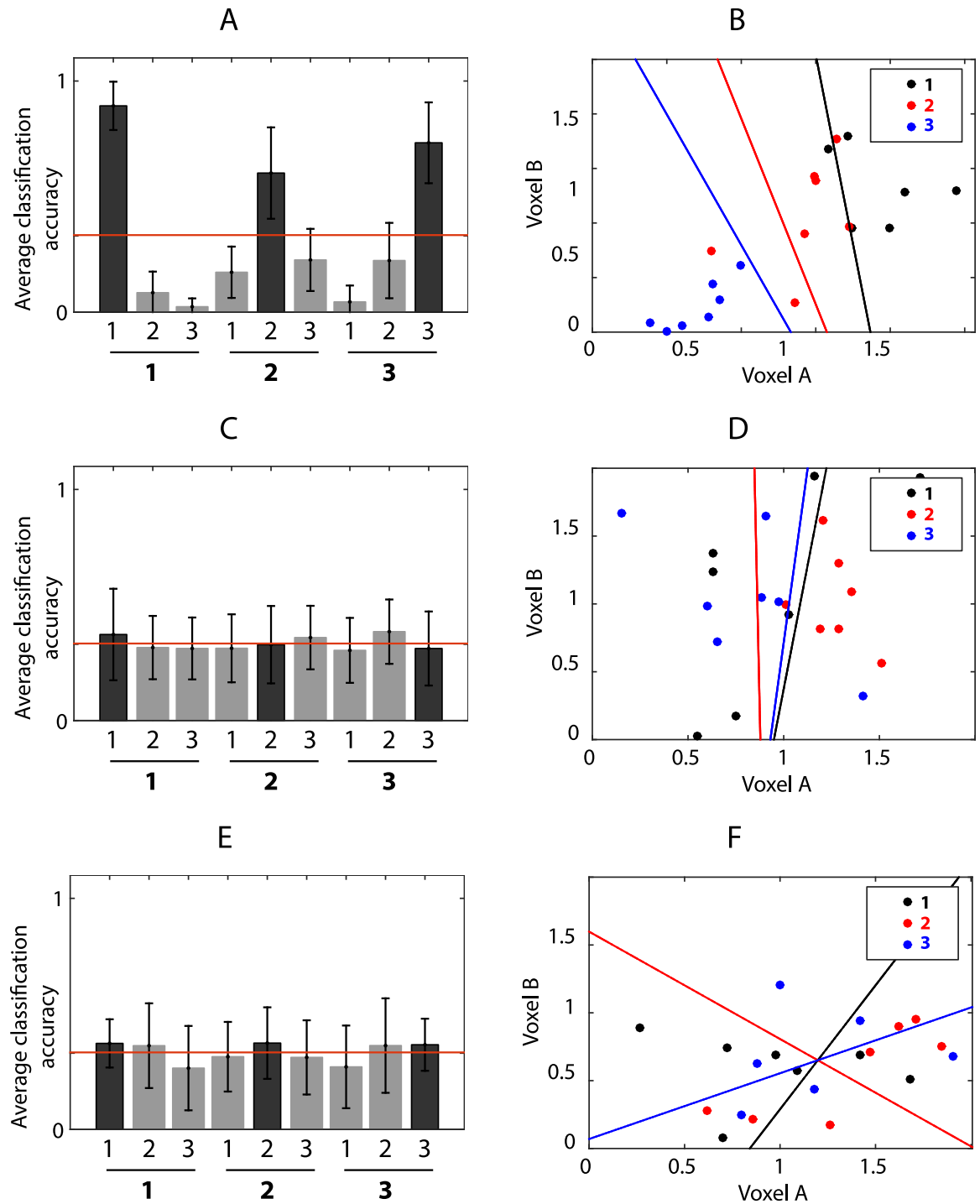
Fig 4. LDA of item position in V1 using different subsets of voxels. Top row: all voxels from V1; middle row: only retinotopically activated voxels from V1; bottom row: only retinotopically suppressed voxels from V1. Left column: Bar charts display the average classification accuracy across participants by comparing the known positions (labels) to the predictions made by the classification algorithm. Bars show the proportion of predicted values for each position. Correct classifications are represented with a darker bar. Error bars show the standard error of the mean. The red line depicts the chance level classification accuracy 1/3. Right column: LDA between-class boundaries based on two voxels from the set. Data from [33].
