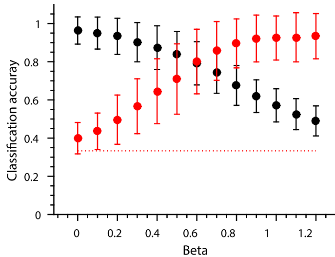
Fig 12. Linear classification accuracy of item identity (black) and position (red) as a function of additive interference (as represented by the \beta parameter, Eq (4)). The red dotted line shows chance level classification accuracy. Error bars depict SEM based on 1,000 simulations of the interference process with fixed parameter values.
