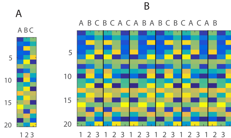
Fig 5. Simulated responses to items. (A) Item patterns over 20 voxels. (B) Six sequences as permutations of three items. Item codes are displayed on the top of x-axis, position codes at the bottom.
