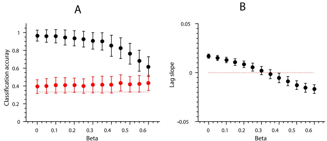
Fig 15. Classification accuracy and positional similarity as simulated by the proportional interference mechanism. Error bars depict SEM based on 1,000 simulations of the interference process. Notice that \beta values on the x-axis have been approximately halved since the parameter now indicated the proportion of residual activity. (A) Linear classification accuracy of item identity (black) and position (red) as a function of proportional interference ( \beta ). The red dotted line shows chance level classification accuracy. (B) The size of the positional lag effect as a function of proportional interference ( \beta ).
