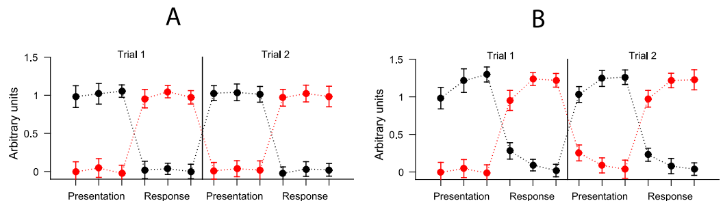
Fig 17. The average simulated activity of two sets of voxels, each sensitive either to the presentation or recall phase of the task. In this hypothetical task a presentation of three items in a sequence is followed by recall of three items. (A) Without interference. (B) Additive interference.
