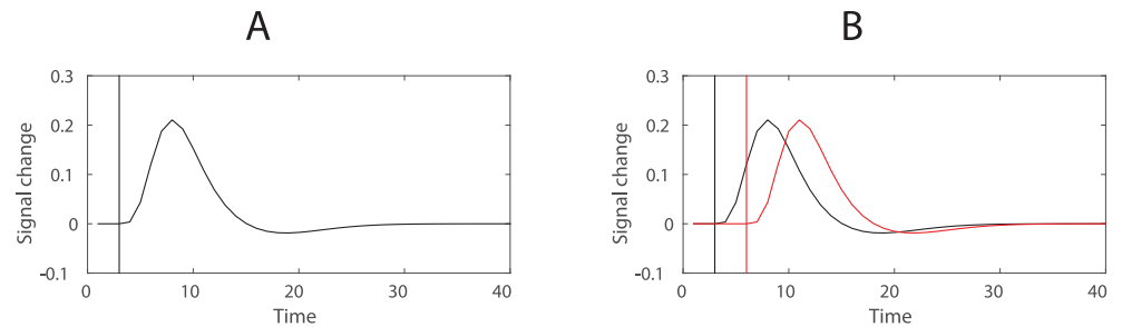
Fig 18. Temporal interference in fMRI. (A) The haemodynamic response function (HRF) with the vertical line representing the corresponding neural event. (B) Temporal interference between two adjacent events: black and red lines.
