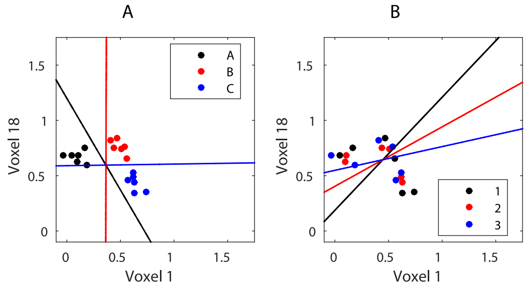
Fig 6. The scatter of item patterns and LDA between-class boundaries based on the two most informative voxels. (A) Item information. (B) Position information.
