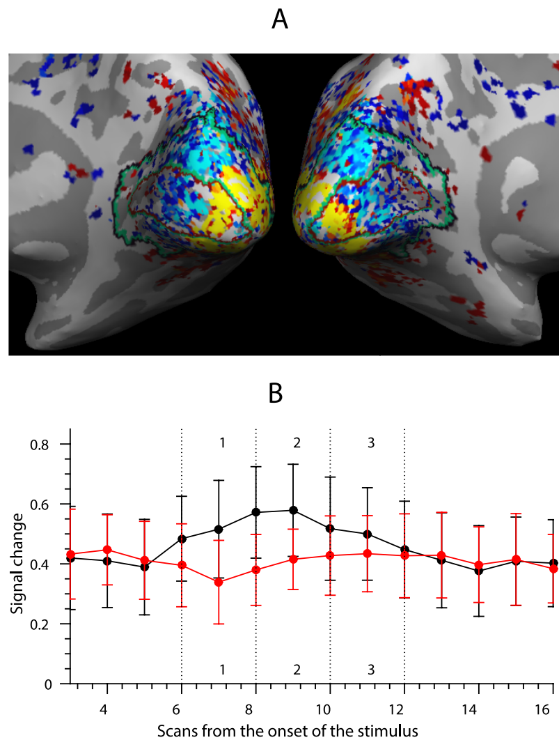
Fig 3. Interference between task phases: Retinotopic suppression. (A) Activation and suppression in V1 averaged across all stimuli for a single participant. The activated voxels (yellow, p < 0.001 ) mark the foveal part of the visual cortex driven by the stimuli (presented at 6° visual angle). (B) Peristimulus time histogram of sequence presentation of two groups of voxels from a single participant's V1. The black line denotes the average of the voxels activated by the stimuli and the red line denotes the average of the voxels suppressed by the stimuli. Dashed vertical lines indicate the time bins where sequence items were presented.
