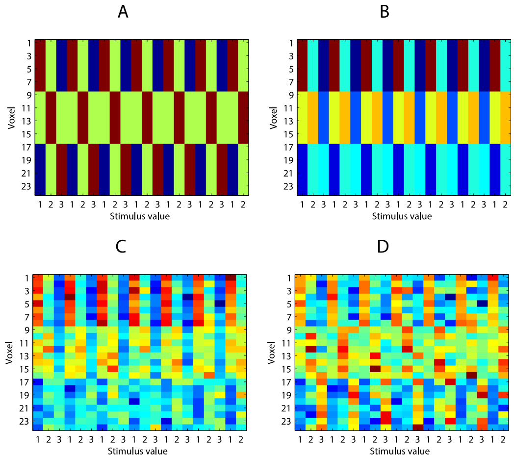
Fig 9. Simulation of sensory adaptation. (A) Voxel response matrix based on positional preferences. (B) Voxel response matrix: positional preferences + sensory adaptation. (C) Voxel response matrix: positional preferences + sensory adaptation + Gaussian noise. (D) Voxel response matrix z-scored. Column-wise means are zero.
