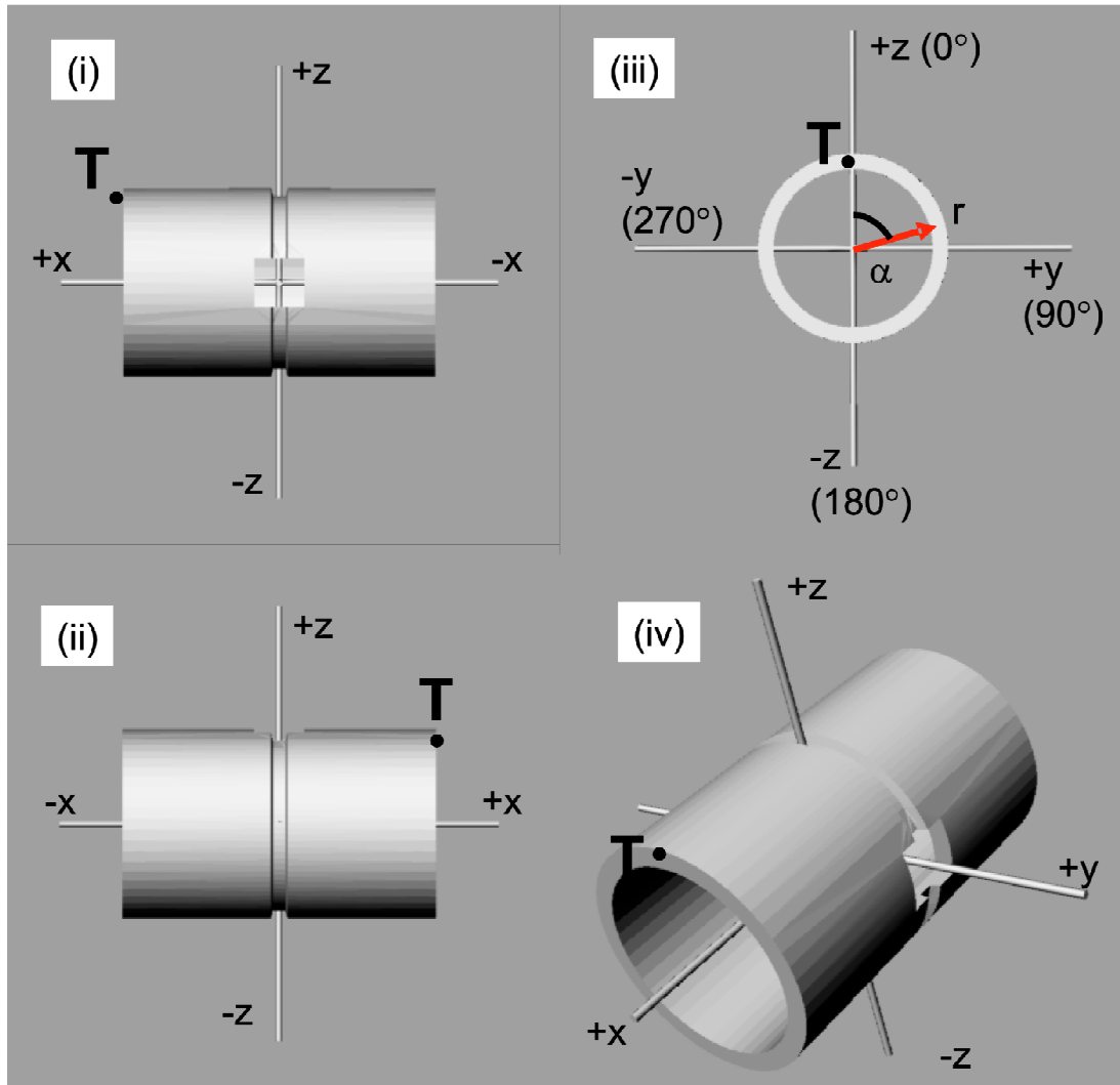
Fig.2. (i) Autogenous pipe weldment relative to Cartesian coordinate system ( x,y,z ) with origin at the centre of the pipe weldment. The view along negative y shows the position of the neutron access aperture. The reference point top dead centre (TDC) is marked with a capital T. (ii) The view along positive y , opposite to the neutron access aperture. (iii) Plan view of the pipe looking along negative x , with TDC and positive x axis pointing upwards out of the plane of the page. This view shows the radius r and azimuthal angle \alpha . It should be noted that \alpha is taken as positive clockwise when looking along the negative x direction as shown. (iv) Oblique view.
