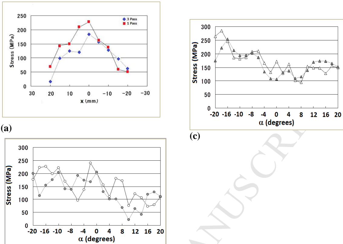
Fig.13. X-ray diffraction measurements. (a) The axial variation of the hoop component of residual stress, measured on the inner surface of the single-pass and triple-pass weldment. (b) The angular variation of the hoop component of residual stress measured on the inner surface of the single-pass weldment, open circles under center of groove at x = 0.0 , and closed circles under first pass at x = + 6.6 mm. (c) The angular variation of the hoop component of residual stress measured on the inner surface of the triple-pass weldment, open triangles under center of groove at x = 0.0 , and closed triangles under first pass at x = + 6.6 mm.
