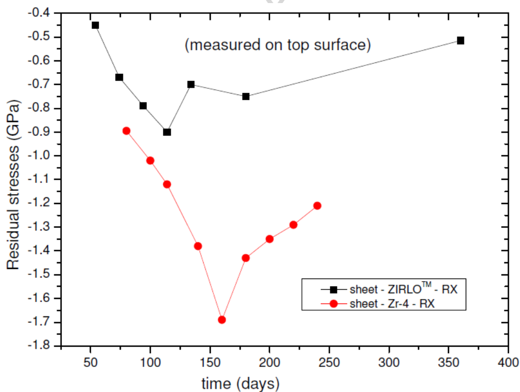
Fig. 5. Raman characterization on the top surface of the oxide grown on sheet ZIRLO RX and Zr-4 RX specimens: (a) Tetragonal phase fraction, and (b) Measured stress profile.
