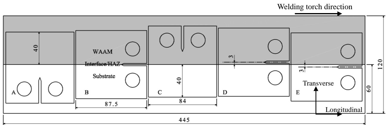
Fig. 1 Layout of test specimens on a WAAM-substrate wall showing the WAAM-substrate interface location on each type of C(T) specimen (unit: mm)
