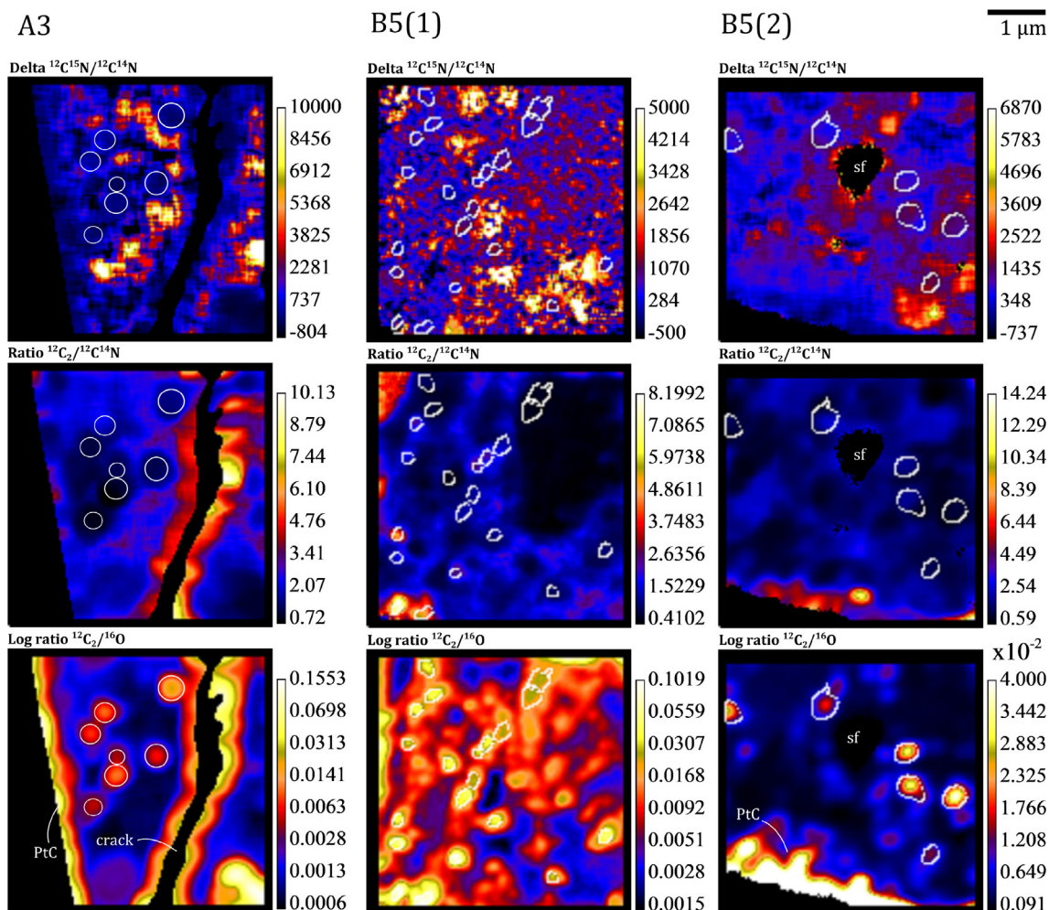
Fig. 6. NanoSIMS raster images for \delta^{15}\text{N} , ^{12}\text{C}_2^-/^{12}\text{C}^{14}\text{N}^- and ^{12}\text{C}^-/^{16}\text{O}^- from three rasters in B5(1), B5(2) and A3. Areas with high ^{12}\text{C}^-/^{16}\text{O}^- ratios represent nanoglobules. These ROIs are overlaid on \text{C}^-/\text{CN}^- and \delta^{15}\text{N} images in white. sf = iron sulfide.
