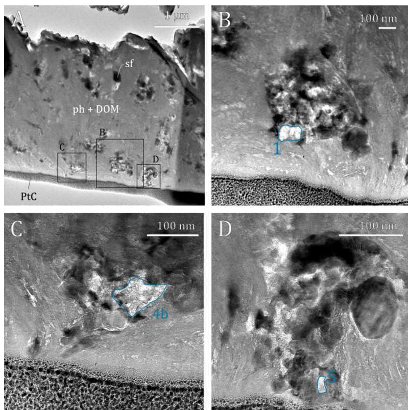
Fig. 5. BFSTEM images from H-clast FIB-section A3. Panel A represents an overview of the section, showing abundant Fe-sulfides (sf) and large phyllosilicate structures. The squares in panel are various zoom-ins of carbonaceous clusters (B–D) that include locations of EELS analyses (blue boundaries, Fig. 7).
