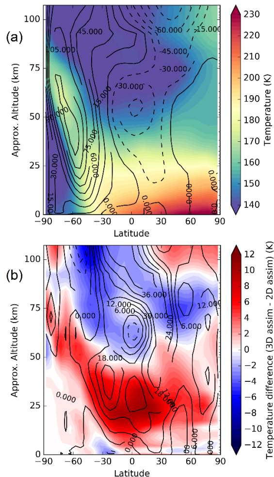
Figure 1: (a) Assimilated zonally averaged temperature and zonal wind speed around L_S 90 for the 3D reanalysis and (b) absolute difference in temperature and zonal wind speed between 3D reanalysis and 2D reanalysis over the same time period.
