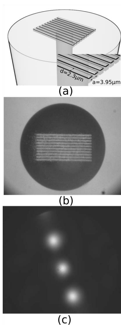
Fig. 2: Scheme of 1-D diffraction grating at fiber end-face with period a=3.95(23) \mu\text{m} and thickness d=2.30(21) \mu\text{m} (a), CCD image of resulting 1-D diffraction grating inscription (b) and its FFP distribution from a 1550 nm laser source (c).
