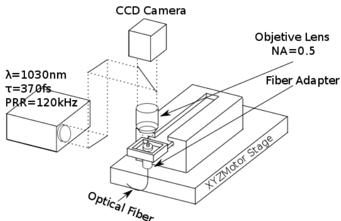
Fig. 1: Set-up diagram for longitudinal and surface writing.
