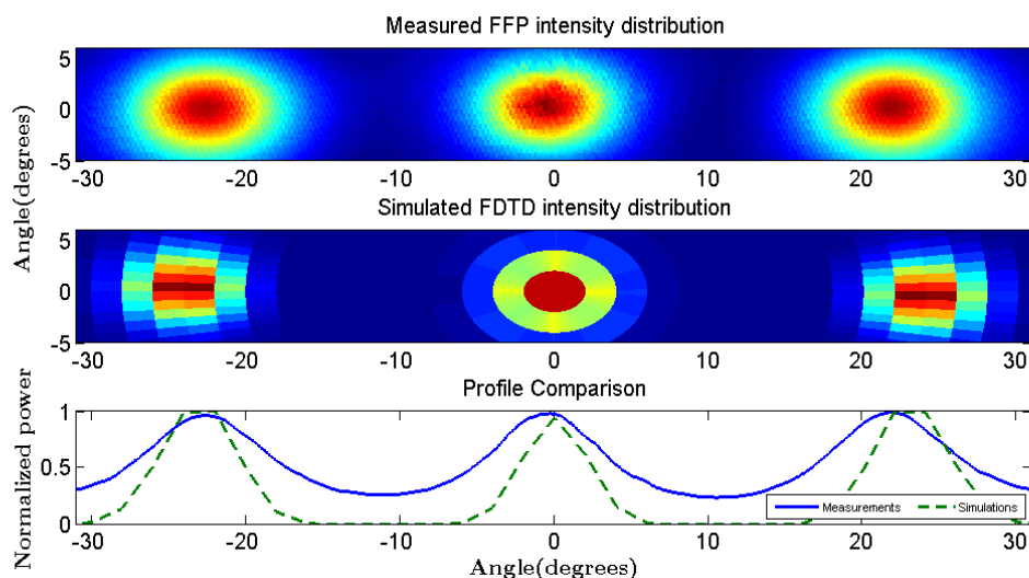
Fig. 3: Angular intensity distribution for FFP measurements and FDTD simulation. Both profiles are compared below.
