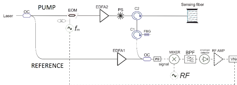
Figure 1. Experimental setup of BOFDR system. EOM: electro-optic modulator. OC: optical coupler; PS: polarization scrambler; PD: photodetector; BPF: electrical bandpass filter.
