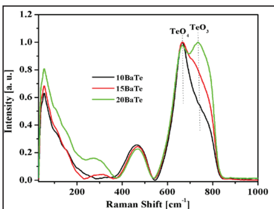
FIGURE 4. Raman spectra of BaO- \text{TeO}_2 glasses.
