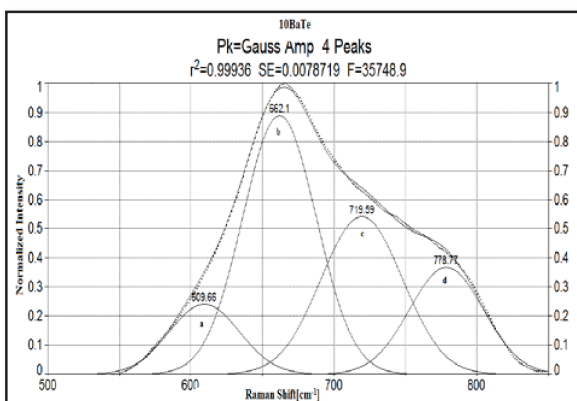
FIGURE 4. Raman spectra of BaO- \text{TeO}_2 glasses.
