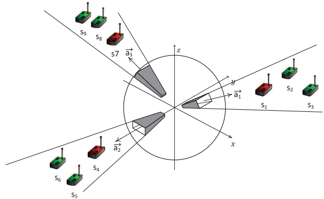
Fig. 3. Antenna distribution in 60 GHz energy harvesting
