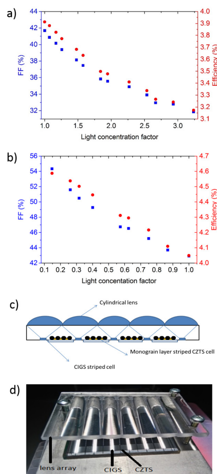
Figure 4: FF and efficiency revealing CZTS solar cell performance under a) enhanced and b) reduced illumination conditions; c) schematic and d) prototype of combined CIGSe-CZTS direct-diffuse micro concentrator concept.
