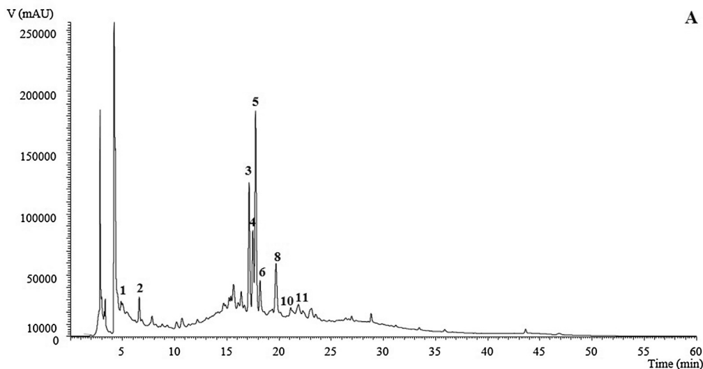
Fig. 1. HPLC chromatogram of OG phenolic profile recorded at 370 nm (A), betaxanthins profile of OS recorded at 484 nm (B) and betacyanins profile of OE recorded at 535 nm (C).
