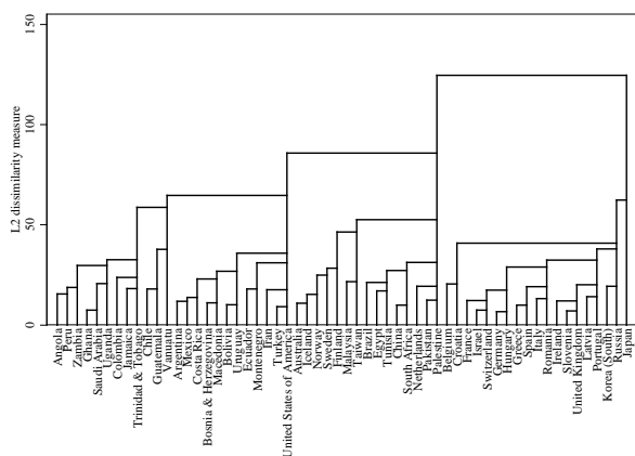
Fig. 2. Complete linkage dendrogram.
