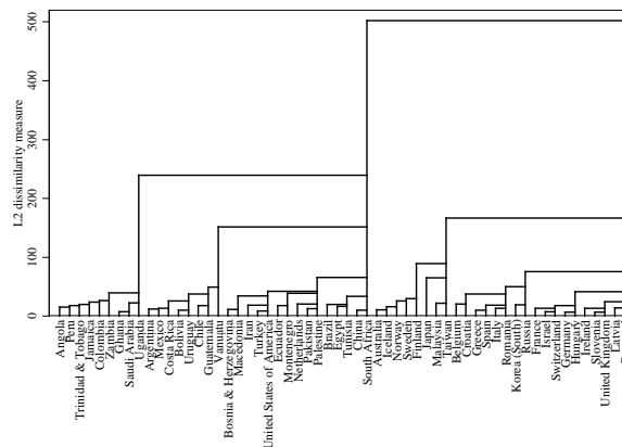
Fig. 3. Ward's linkage dendrogram.
