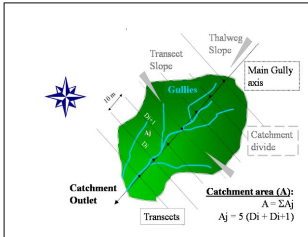
Figure 6: Field measurements for estimating catchment geometry.
