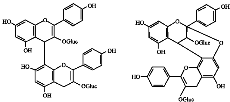
Fig. 5: Suggested structures for compound e ( m/z at 865)
