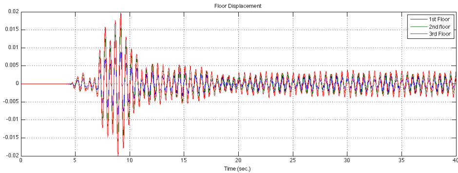
Figure 31. Kobe - Uncontrolled response
