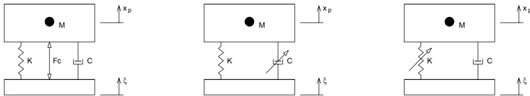
Figure 1. Active and semi-active vibration control strategies
