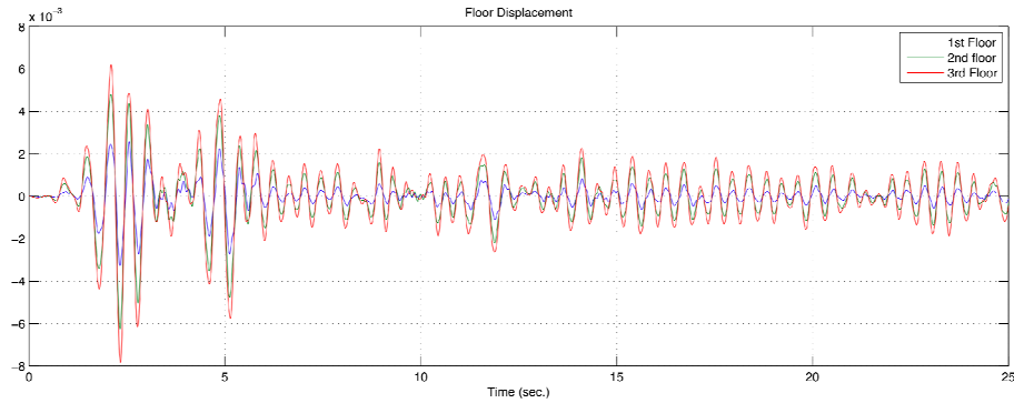
Figure 28. El Centro-Uncontrolled response with MR damper @0.0A (passive ON)
