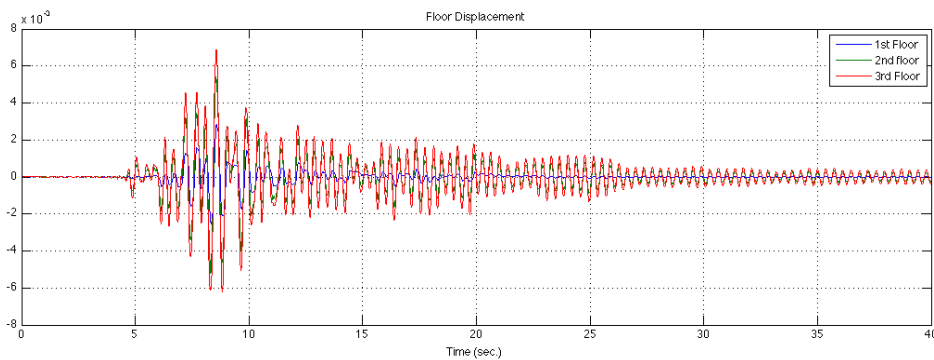
Figure 33. Kobe-Uncontrolled response with MR damper @0.25A (passive ON)
