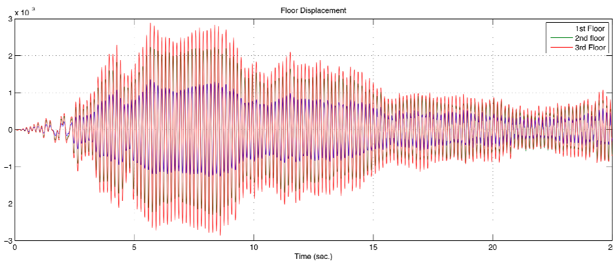
Figure 30. El Centro-Controlled response with MR damper (semi-active ON)
