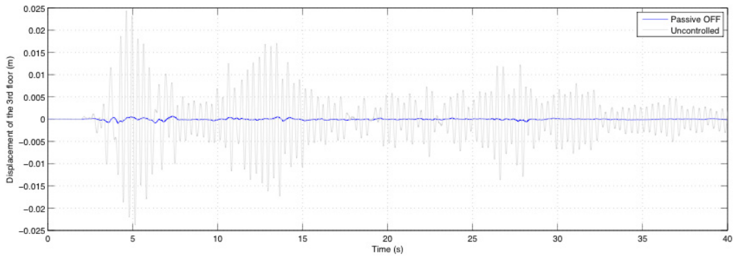
Figure 25. Displacement of the 3rd floor with semi-active control
