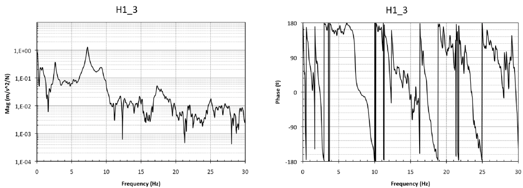
Figure 19. FRF magnitude and phase of H1_3 with MR damper at 0.0A
