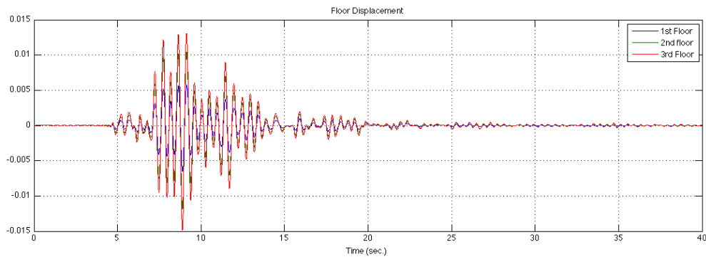
Figure 32. Kobe-Uncontrolled response with MR damper @0.0A (passive ON)
