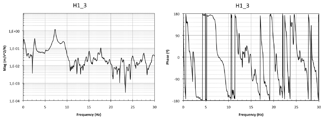
Figure 22. FRF magnitude and phase of H1_3 with MR damper at 0.5A
