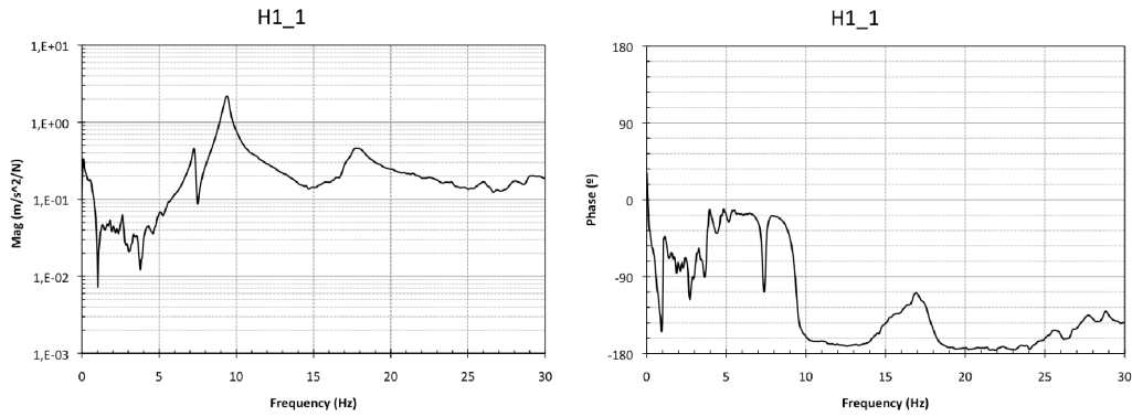
Figure 20. FRF magnitude and phase of H1_1 with MR damper at 0.5A
