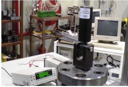
Figure 6. Magneto-rheological damper RD-1005-03 test setup at FEUP
