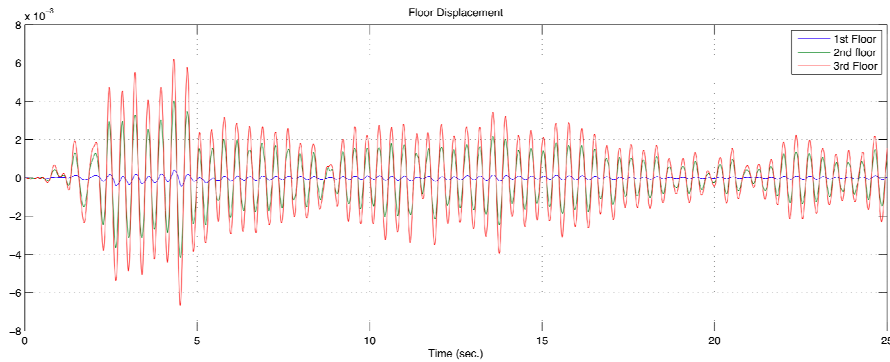
Figure 29. El Centro-Uncontrolled response with MR damper @0.25A (passive ON)
