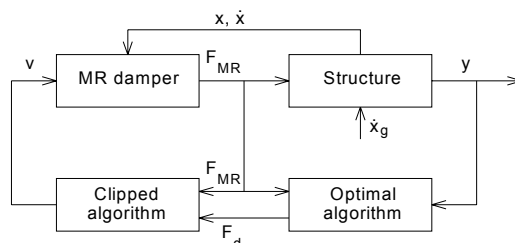
Figure 5. Clipped Optimal controller for a MR damper
