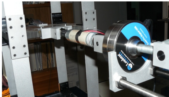
Figure 16. MR damper and load cell
