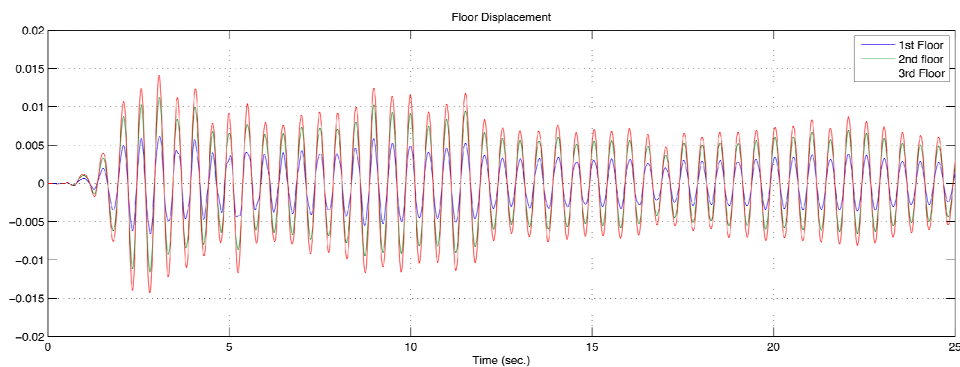
Figure 27. El Centro - Uncontrolled response
