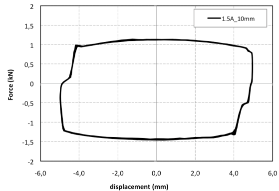
Figure 8. MR damper RD-1005-03 Force-Displacement curves (1.5 A , 10mm)
