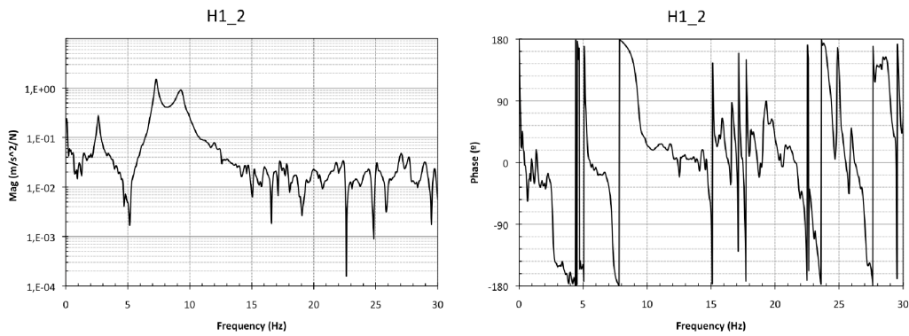
Figure 21. FRF magnitude and phase of H1_2 with MR damper at 0.5A
