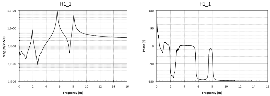
Figure 13. FRF magnitude and phase of H1_1
