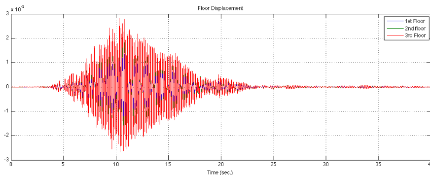
Figure 34. Kobe-Controlled response with MR damper (semi-active ON)
