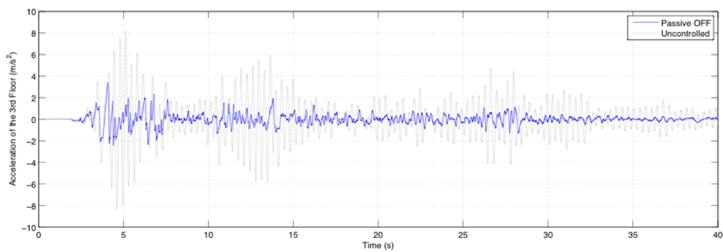
Figure 26. Acceleration of the 3rd floor with semi-active control
