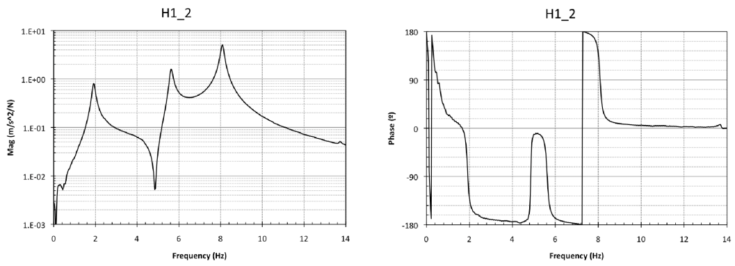
Figure 14. FRF magnitude and phase of H1_2
