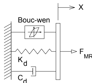
Figure 3. Bouc-Wen model for a MR damper
