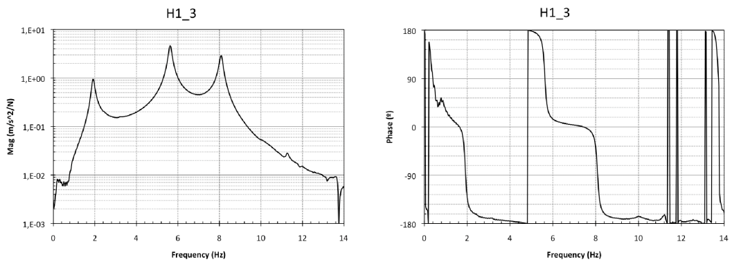
Figure 15. FRF magnitude and phase of H1_3
