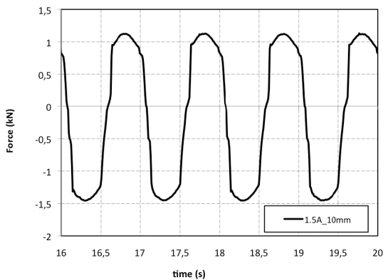
Figure 7. MR damper RD-1005-03 Force-Time History (1.5 A , 10mm)
