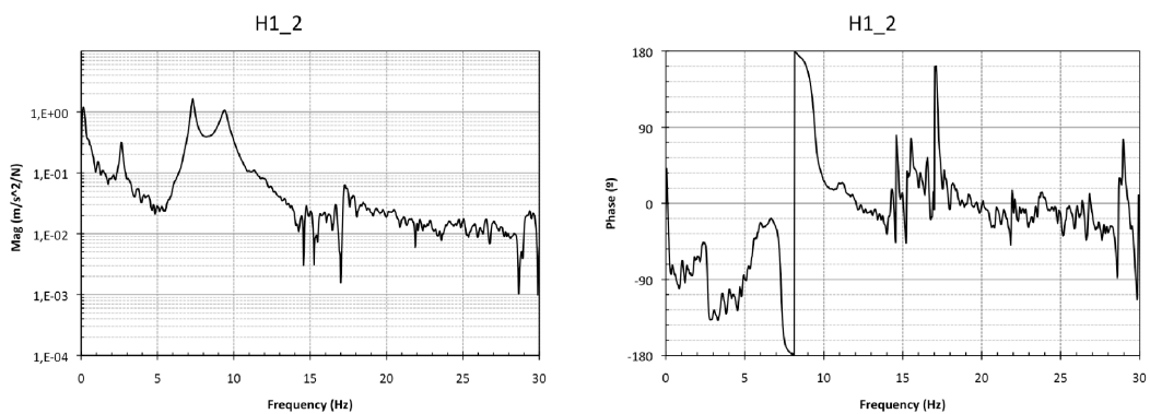
Figure 18. FRF magnitude and phase of H1_2 with MR damper at 0.0A
