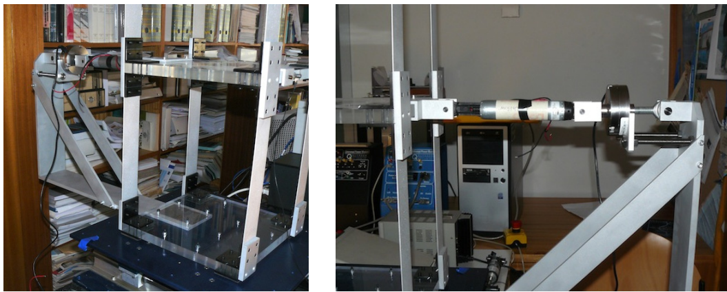
Figure 10. MR damper attached to the experimental metallic frame
