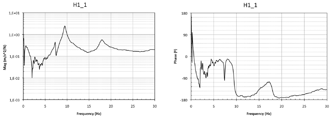
Figure 17. FRF magnitude and phase of H1_1 with MR damper at 0.0A
