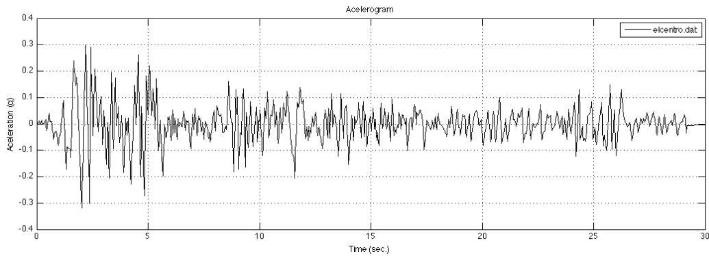
Figure 23. El Centro earthquake signals for semi-active control (Lyapunov and Clipped-Optimal)
