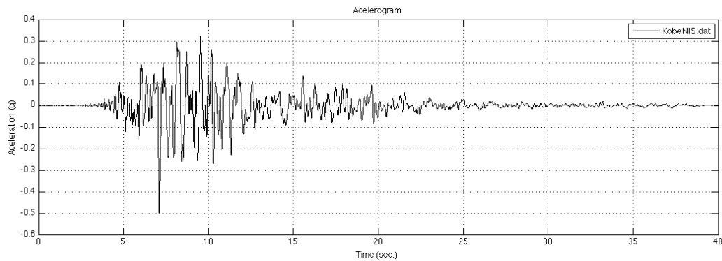
Figure 24. Kobe NIS earthquake signals for semi-active control (Clipped-Optimal)
