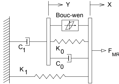
Figure 4. Modified Bouc-Wen model for a MR damper
