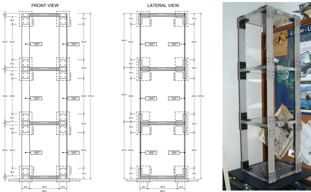
Figure 9. Geometrical properties and perspective view of the scaled frame (FEUP)
