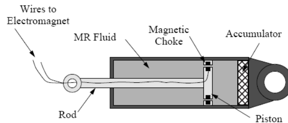
Figure 2. Schematic representation of a magneto-rheological damper
