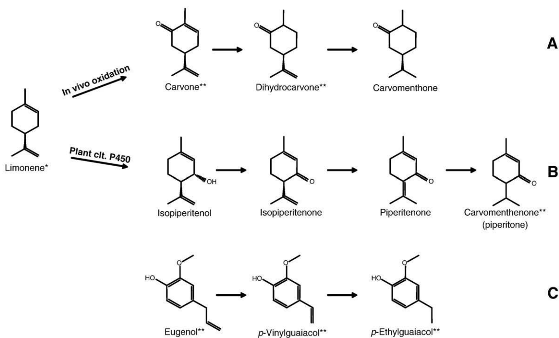
Fig. 4. Possible pathway to the obtainment of carvone, dihydrocarvone and carvomenthone from limonene (A). Biosynthesis of carvomethenone in Mentha piperita (B). Obtainment of p -vinylguaiacol and p -ethylguaiacol from eugenol (C).
