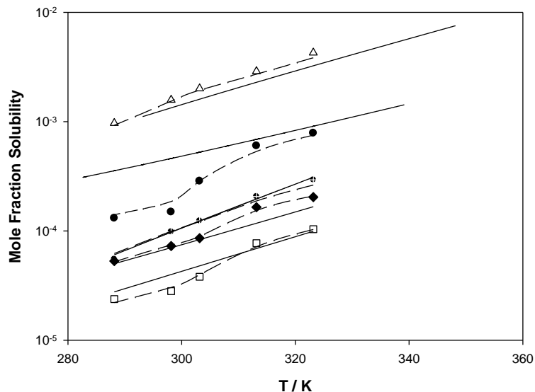
Figure 1: Experimental solubility data (●, salicylic acid; Δ, gallic acid; □, trans-cinnamic acid; ⊕, caffeic acid; ◆, ferulic acid) and modelling results by CPA (solid line) and UNIQUAC (dotted line).
