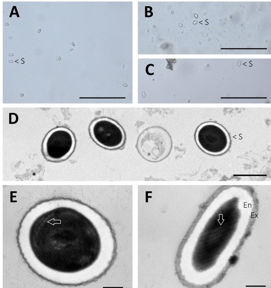
Fig. 2. In A: Light micrographs of spores (S) of Nosema neumanni n. sp. which seem slightly smaller than spores of Nosema ceranae (in B) and Nosema apis (in C). In D, E and F: electron micrographs of spores of Nosema neumanni n. sp. with electron dense exospore (Ex) and electron lucent endospore (En). Spore size measurements under transmission electron microscopy confirms that spore length ( 2.36 \pm 0.14 \mu\text{m} ) and width ( 1.78 \pm 0.06 \mu\text{m} ) is smaller than of the two already known Nosema spp. associated with honeybees. Moreover, Nosema neumanni n. sp. has fewer filament coils (10–12; white arrows). Scale bars: in A, B and C 50 \mu\text{m} ; in D 2 \mu\text{m} and in E and F 500 nm.
