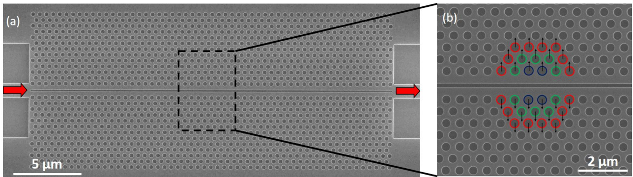
Figure 1 (a). SEM image of air-slot cavity, (b) zoomed in SEM image of slot cavity highlighting the shifting of holes denoted by the black arrows (red: 5 nm; green: 10 nm; blue: 15 nm).
