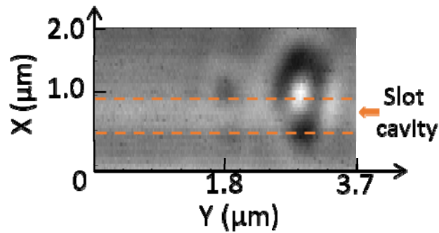
Figure. 4. Map of the intensity variation induced by the interaction between the nano-tip fiber and the air-slot cavity.
