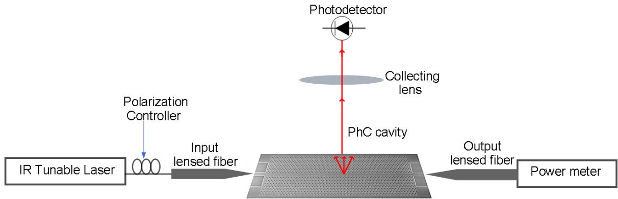
Figure 2. Schematic of the experimental apparatus used for characterize PhC cavity.
