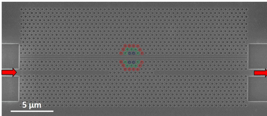
Figure 5. SEM image of side-coupled air-slot cavity.
