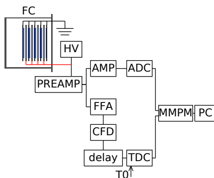
(b) DAQ for the fission chamber (FC). HV: high voltage supplier, PREAMP: charge-integrating preamplifier, AMP: spectroscopy amplifier, ADC: analogue-to-digital converter, FFA: fast filter amplifier, CFD: constant fraction discriminator, TDC: time-to-digital converter, MMPM: multiplexer.
