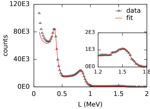
Figure 3.14: Experimental (“data”) and modelled (“fit”) spectra for the ^{207}\text{Bi} source, for an EJ301 detector.
