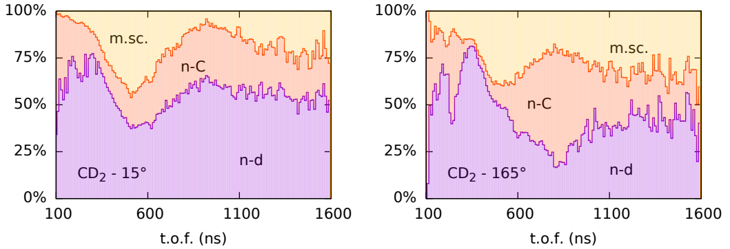
Figure 6.8: Contribution of multiple scattering in the target (“m.sc.”), single scattering on deuterium (“n-d”) or on carbon (“n-C”), expressed in percentage of number of events as a function of the time of flight.
