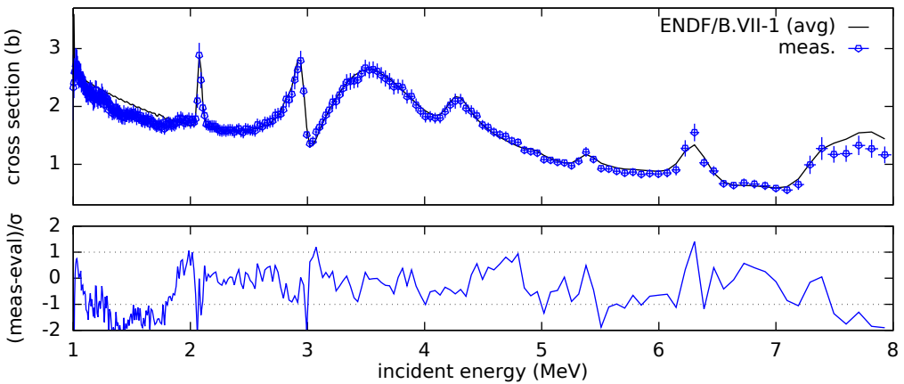
Figure 4.12: Elastic scattering cross section: the measurements are compared to the evaluation averaged according the experimental energy resolution (“ENDF/B-VII.1 (avg)”). The deviation of the experimental data from the evaluated cross section, expressed as the difference between measurement and evaluation ( meas-eval ) divided by the experimental uncertainty ( \sigma ), is also shown as a function of the neutron incident energy.
