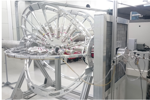
(a) Picture of the setup installed in the measurement station at 108^\circ , 30 m distance from the GELINA neutron source. The neutron beam comes from the right; it first passes through the fission chamber, then hits the target at the centre of the scintillator array. The fission chamber is mounted on a lead wall which is the last collimator (at 25.8 m distance from the source) shown in figure 3.2.
