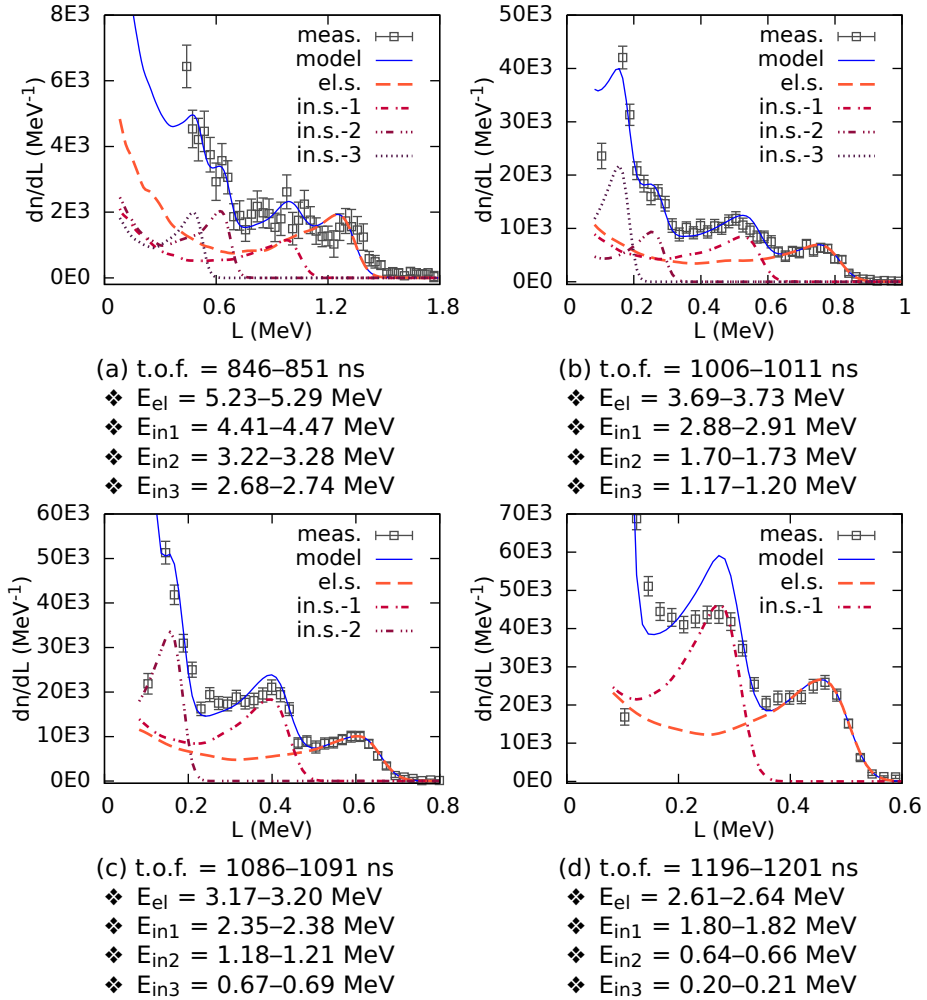
Figure 5.4: Same as figures 5.3, but for an EJ315 detector. The detection threshold for this detector is 90 keV in electron energy, which corresponds to 655 keV in neutron energy.
