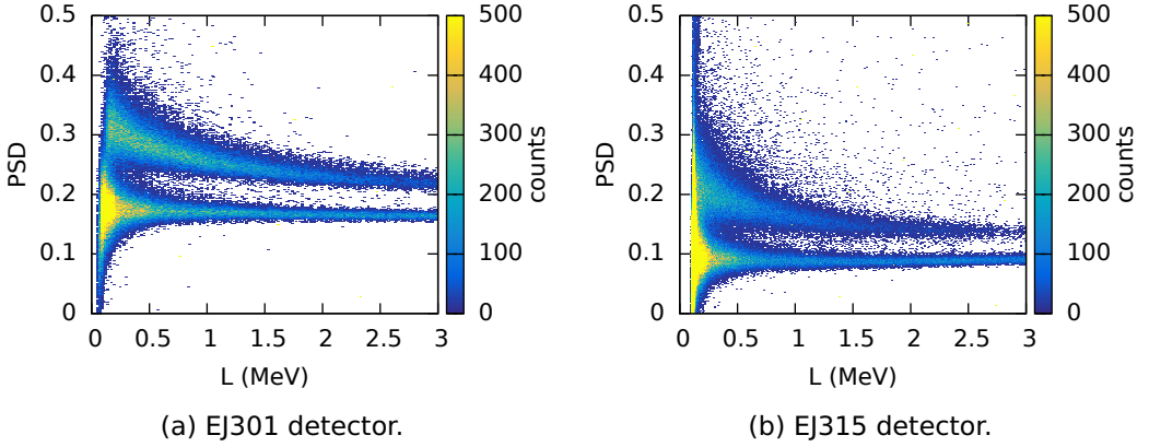
Figure 3.8: Two-dimensional histograms representing the PSD distribution as a function of the light output L . The data taken during a measurement with an AmBe source are shown for one of the EJ301 and one of the EJ315 detectors.
