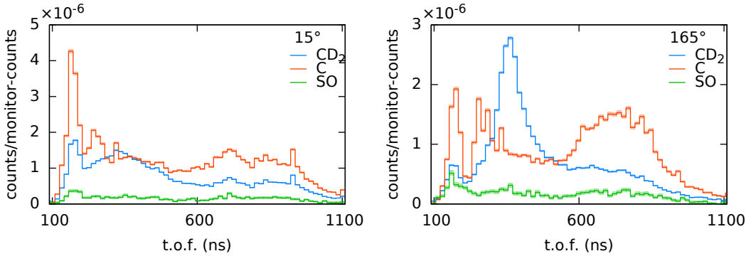
Figure 6.6: Example t.o.f. histograms, one for a detector at 15^\circ and one at 165^\circ , after the room background subtraction. The counts have been normalized with the monitor counts for proper comparison between the \text{CD}_2 , sample-out (SO) and graphite (C - carbon) measurements.
