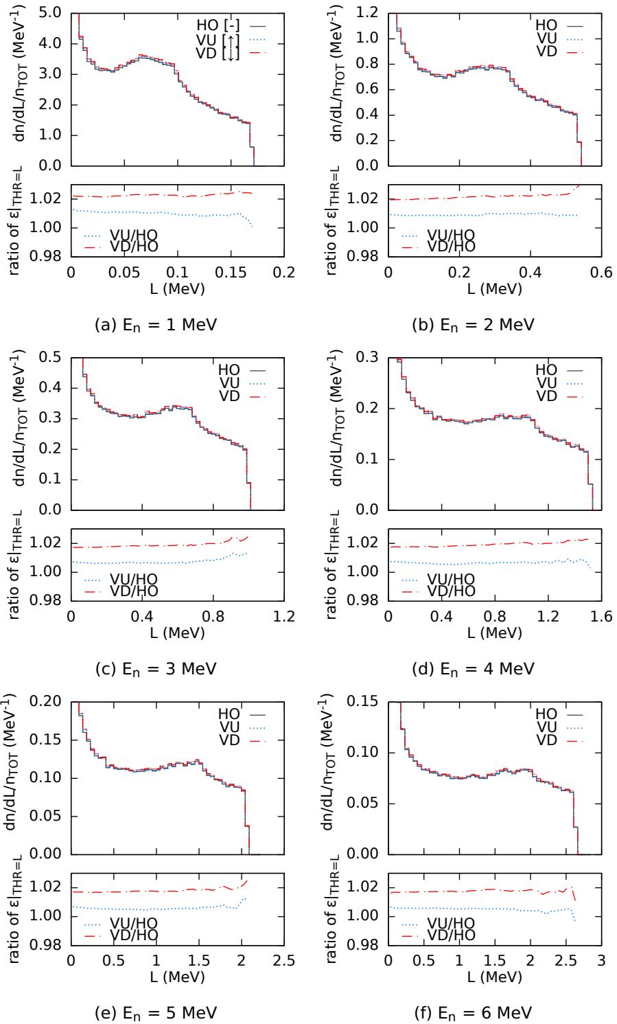
Figure 3.21: Differences in the EJ301 neutron response and efficiency caused by placing the detector in different orientations. “HO”: detector in horizontal; “VU”: detector in vertical, facing upwards; “VD”: detector in vertical, facing downwards. The light output distributions per total number of neutrons entering the detector dn/dL/n_{TOT} and the ratio of the efficiency as a function of the threshold \varepsilon|_{THR=L} of the vertical detectors to the horizontal detector are shown.
