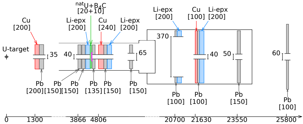
Figure 3.2: Scheme of the collimation for the flight path at 108^\circ . The collimation system consists of a set of pierced disks made of lead, copper and lithium epoxy (“Li-epx”) of variable thickness (in square brackets) and with different internal diameter. Two filters are used: a natural uranium filter (for photons) and a boron filter (for slow neutrons). The axis below the figure indicates the distance of the collimators and filters to the neutron producing targets. All dimensions are given in millimetres.
