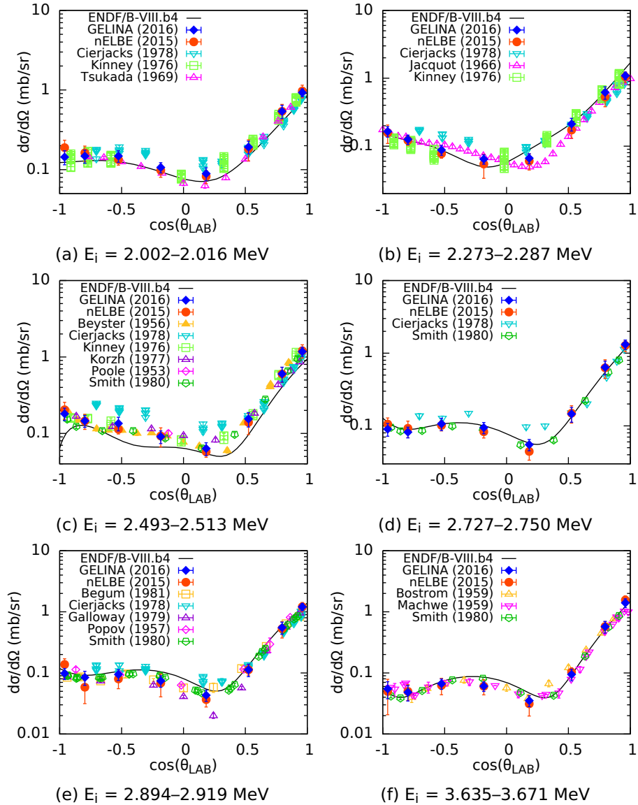
Figure 5.5: Differential cross section d\sigma/d\Omega of neutron elastic scattering on natural iron as a function of the cosine of the scattering angle in the laboratory system \theta_{LAB} , for selected intervals of incident neutron energy E_i . The results of the measurements at GELINA and nELBE are compared with the measurements from the EXFOR database and the angular distribution reported in the ENDF/B-VIII.b4 library (CIELO evaluation).
