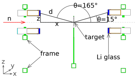
Figure 6.3: Model of the detectors, the target, and the supporting aluminum frame implemented in MCNP5. Here the vertical x - z plane passing through the center of the target is shown; an analogous figure is obtained when the x - y plane is plotted, with the difference that there the distance z is replaced by that along the y -axis. The distances x , y , and z were actually measured, d and the angle \theta were computed accordingly. The exact values of x , y or z , d , and \theta are reported in Table 6.3.
