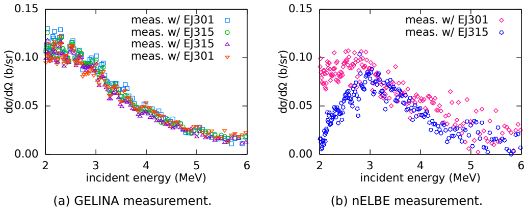
Figure 5.9: Differential cross section d\sigma/d\Omega of neutron inelastic scattering from the first excited level of ^{56}\text{Fe} as a function of the neutron incident energy. The results obtained at 121.7^\circ are shown for each detector separately (the scintillator type is indicated in the graph). The points are shown without uncertainties to improve the readability of the plot.
