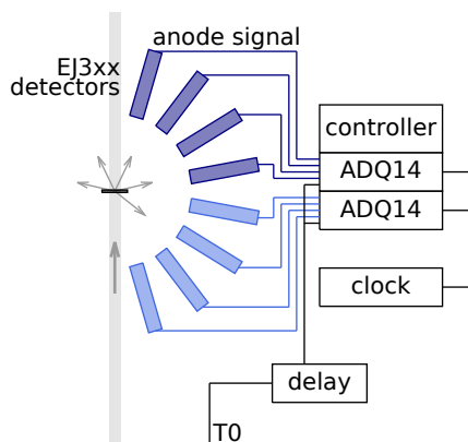
(a) DAQ diagram for one set of 8 scintillation detectors. The full DAQ system consists of 8 ADQ14 digitizer cards: they are all installed on the same PXIe chassis, managed by the same controller PC and the synchronization is performed using one clock generator for all cards.
