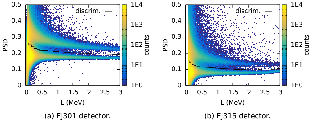
Figure 4.3: Two-dimensional histograms representing the events recorded by an EJ301 detector and an EJ315 detector arranged according to the signal light output L (in equivalent electron energy) and the Pulse Shape Discrimination factor PSD . The segmented line (“discrim.”) represents the “optimal” separation point between neutrons and photons found applying equation (4.3) in the light output interval subtended by each segment.
