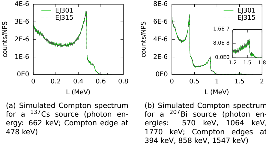
Figure 3.12: Light output spectra simulated with MCNP for EJ301 and EJ315 detectors with infinitesimal resolution, using photon sources. The number of pulses generated per photon (counts per starting particle, NPS) is represented as a function of the electron light output.
