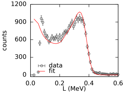
(a) Detector at 163.8^\circ ❖ t.o.f. = 1131–1136 ns ❖ E_i = 3.06\text{--}3.09 MeV ❖ E_n = 2.20\text{--}2.22 MeV ❖ E_{n,\text{simul}} = 2.2 MeV
