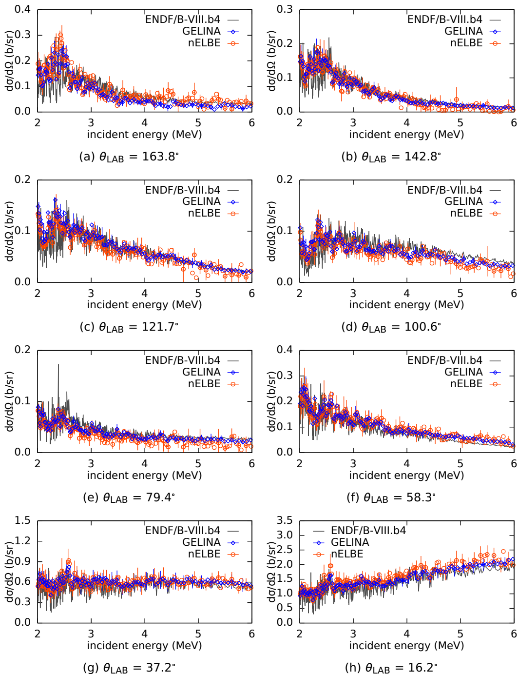
Figure 5.6: Differential cross section d\sigma/d\Omega of neutron elastic scattering on natural iron as a function of the neutron incident energy: comparison of the measured values with the CIELO evaluation from the ENDF/B-VIII.b4 nuclear data library at the laboratory angles \theta_{\text{LAB}} . To improve the readability of the graphs, the experimental uncertainties are given every three points.
