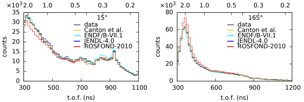
Figure 6.16: Comparison the experimental t.o.f. spectra with the MCNP5 simulations obtained after using several different libraries for the deuterium cross section tables. These spectra are the sum of the counts coming from all detectors at same angle.
