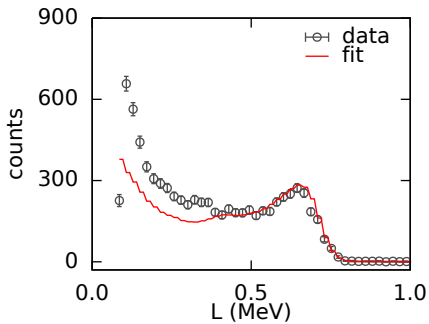
(g) Detector at 58.3^\circ ❖ t.o.f. = 1029–1034 ns ❖ E_i = 3.68\text{--}3.72 MeV ❖ E_n = 3.40\text{--}3.43 MeV ❖ E_{n,\text{simul}} = 3.4 MeV
