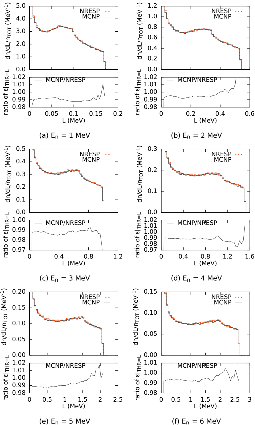
Figure 3.20: Comparison of the unbroadened response function of a NE213 detector computed with NRESP and with MCNP for different neutron energies ( E_n as indicated below each plot). For each neutron energy, the detector response is represented as number of pulses per light output per total number of neutrons entering the detector ( dn/dL/n_{TOT} ). For both models, the efficiency was determined as a function of the threshold ( \epsilon|_{THR=L} ); here the ratio of MCNP to NRESP is shown.
