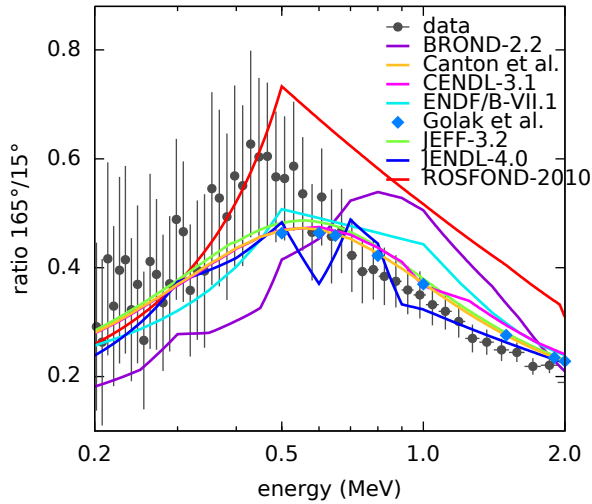
Figure 6.15: Comparison of the ratio \frac{d\sigma}{d\Omega}|_{165^\circ} / \frac{d\sigma}{d\Omega}|_{15^\circ} : experimental results versus the main evaluated libraries and the calculations of Canton et al.
