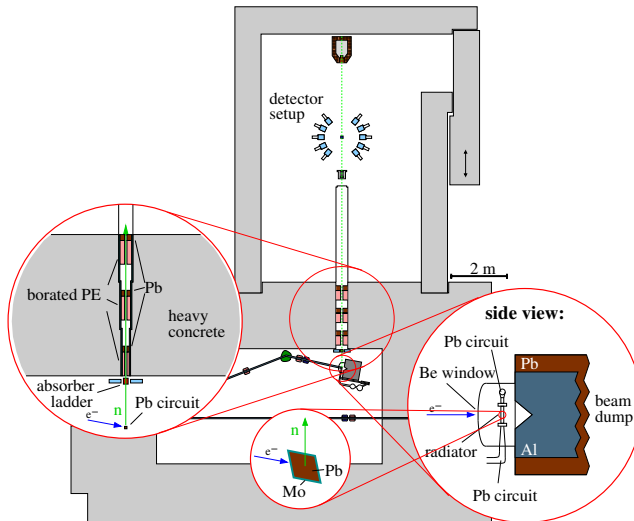
Figure 3.3: Scheme representing the neutron time-of-flight facility nELBE: the electron beam impacts on a liquid lead target confined in a molybdenum channel, the neutron beam is defined by a collimator installed at 95^\circ , and the detector setup is separated from the neutron radiator by a 2.5 m thick wall of heavy concrete.
