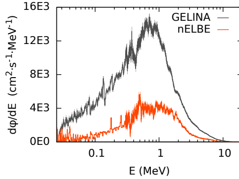
Figure 5.1: Energy distribution d\phi/dE of the neutron flux incident on the iron sample. The flux \phi given here is the average over the measurement time.
