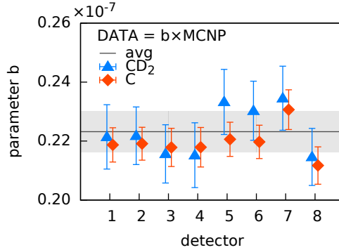
Figure 6.11: Rescaling factor for the MCNP results obtained for each detector (detectors at 15°: numbers 3, 4, 7, and 8; at 165°: 1, 2, 5, and 6), for the CD 2 and graphite (C) runs. The parameter b has an order of magnitude of 10^{-7} because the data were normalized by the monitor counts. The arithmetic average (avg) of all values is what was used to rescale the simulations to the data in Figs. 6.7, 6.9, and 6.12.
