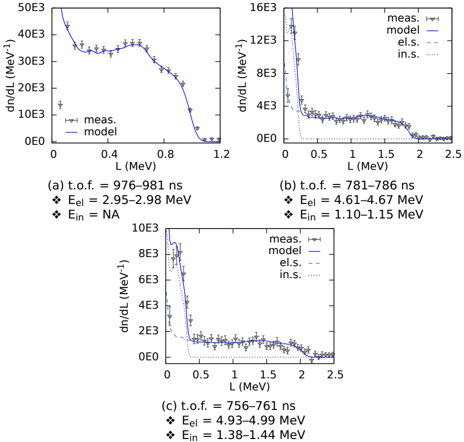
Figure 4.8: Neutron light output distribution ( dn/dL ) measured with an EJ301 detector at 163.8^\circ (“meas.”), compared to the detector response (“model”). The response is the sum of the contribution of elastic scattering (“el.s.”) and of inelastic scattering from the first excited state of carbon (“in.s.”). The experimental light output distributions were obtained gating on the t.o.f. intervals indicated below each figure. E_{el} and E_{in} are the corresponding neutron energies after an elastic (“el”) or inelastic (“in”) collision with carbon.
