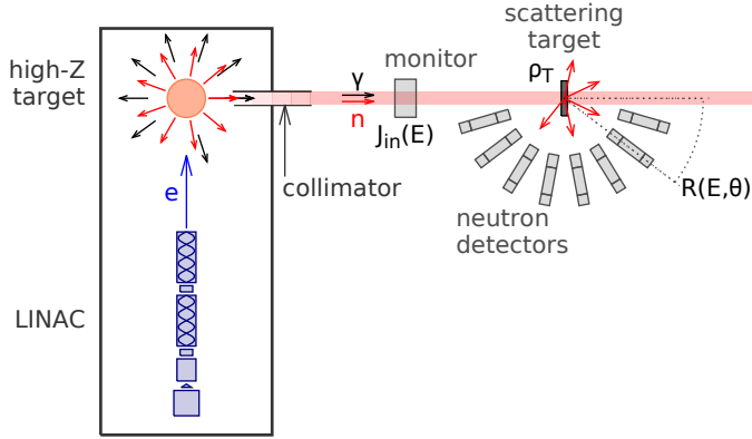
Figure 2.1: General structure of a time-of-flight measurement for the determination of neutron scattering cross sections. The bremsstrahlung photons and the collimated neutron beam, produced by an electron-linac-driven source, strike on a sample of the investigated material, which is characterised by an atomic areal density \rho_T . The incident neutron current J_{in}(E) is measured as a function of the neutron energy E by a monitor placed upstream the target. The other neutron detectors record the scattering reaction rate R(E, \theta) as a function of E and the scattering angle \theta .
