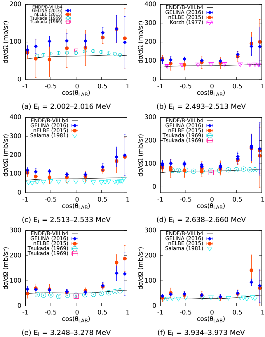
Figure 5.10: Differential cross section d\sigma/d\Omega of neutron inelastic scattering from the first excited level of ^{56}\text{Fe} as a function of the cosine of the scattering angle in the laboratory system \theta_{LAB} , for selected intervals of incident neutron energy E_i . The results of the measurements at GELINA and nELBE are compared with measurements from the EXFOR database and the angular distribution reported in the ENDF/B-VIII.b4 library (CIELO evaluation).
