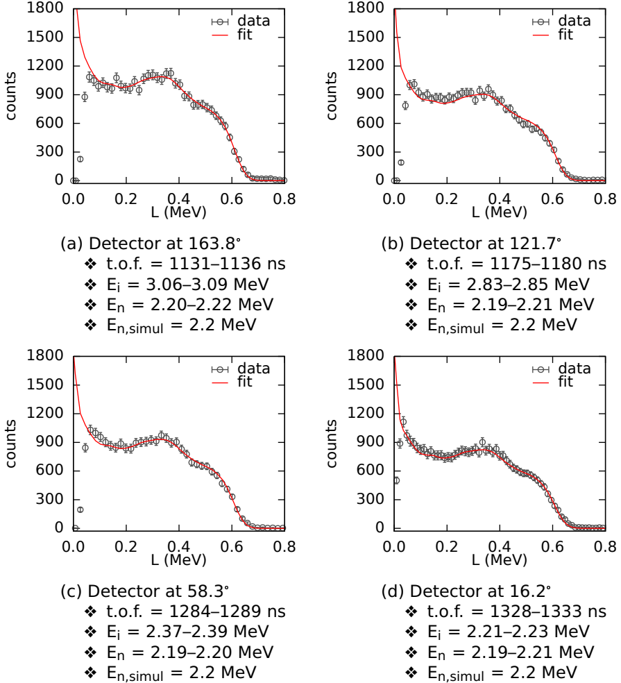
Figure 3.17: Experimental light output histograms (“data”) measured with EJ301 detectors at different angles, compared with the simulated detector responses (“fit”). The histograms represent the light output spectra obtained for neutrons in the t.o.f. intervals indicated below each figure. E_i and E_n are the neutron energy before and after the collision with carbon (elastically scattered neutrons). The detector response functions are modelled for monoenergetic neutrons with energy E_{n,simul} .
