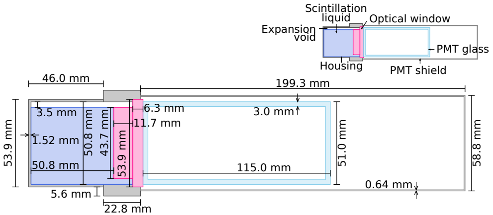
Figure 3.11: Diagram of the MCNP model: the vertical plane passing through the detector axis is shown.
