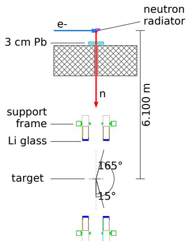
Figure 6.2: Diagram of the experimental setup (horizontal plane passing through the center of the target).
