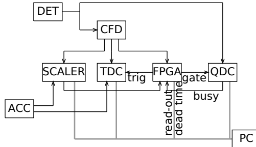
Figure 6.4: Diagram of the data acquisition system. DET: Li-glass detector; ACC: accelerator reference signal; CFD: constant fraction discriminator; FPGA: field programmable gate array logic module; QDC: charge-to-digital converter; TDC: time-to-digital converter; SCALER: scaler module.
