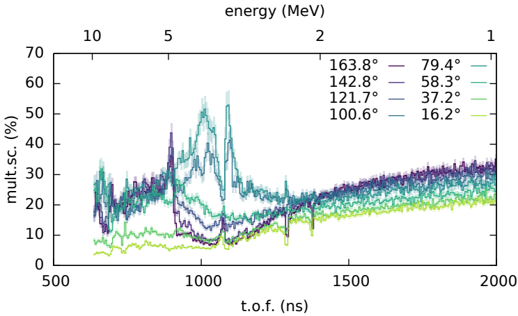
Figure 4.7: Percentage (as a function of the t.o.f.) of events characterised by a neutron colliding multiple times in the graphite target then scattering in the direction of a detector at a given angle. The secondary x-axis gives the incident energy on the target of a neutron scattering elastically to 90^\circ .
