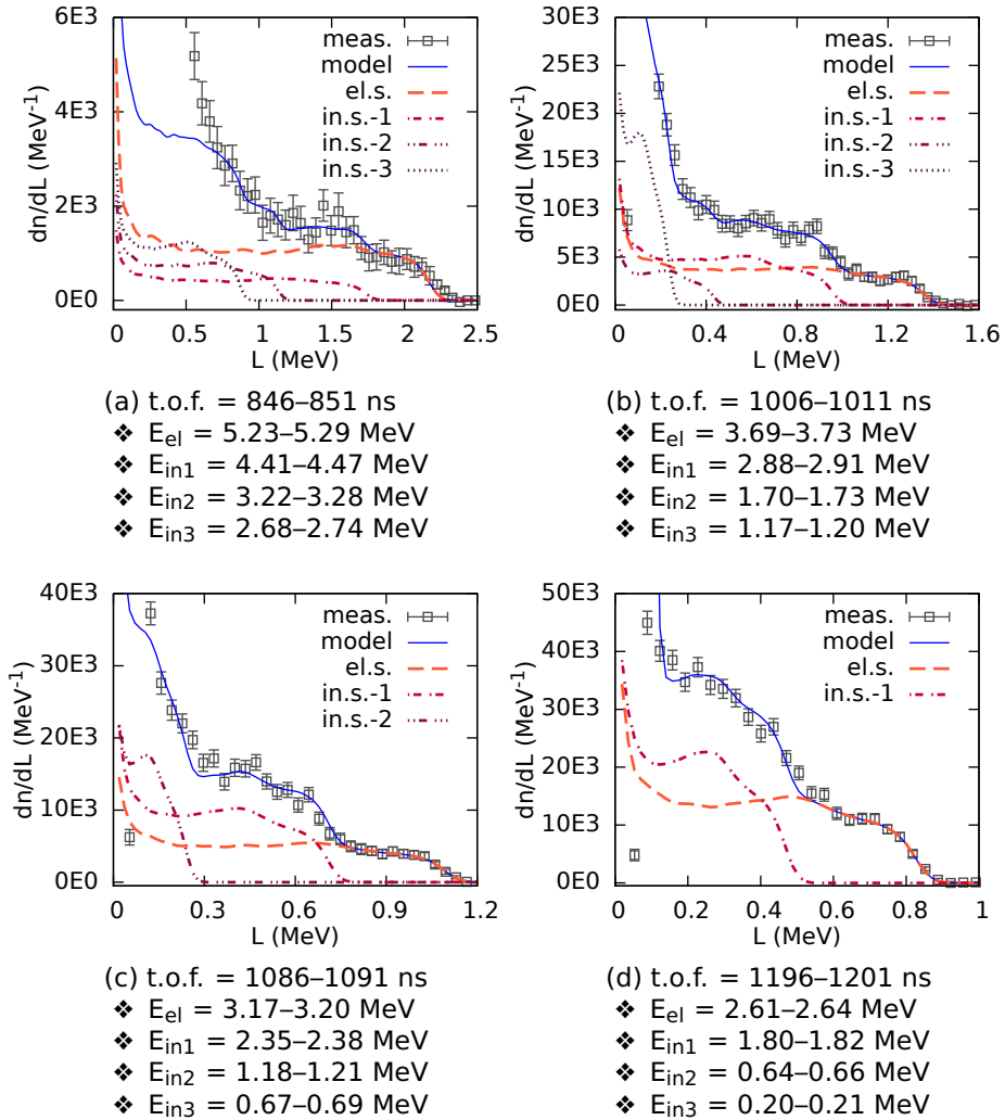
Figure 5.3: Experimental light output histograms (“data”) measured with an EJ301 detector at 100.6^\circ at GELINA (27 m flight path), compared to the simulated detector responses (“model”). The model represents the sum of the contributions of elastic scattering (“el.s.”), and inelastic scattering from the first, second and third excited state of iron (“in.s.-1”, “in.s.-2”, and “in.s.-3”). Below each figure, the t.o.f. interval, and the corresponding neutron energies after an elastic (“el”) or inelastic collision (“in1”, “in2”, and “in3”) are indicated. The detection threshold for this detector is 60 keV in electron energy, or 540 keV in neutron energy.
