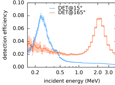
Figure 6.14: Calculated detection efficiency for detectors at 15° and at 165° as a function of the neutron energy incident on deuterium.
