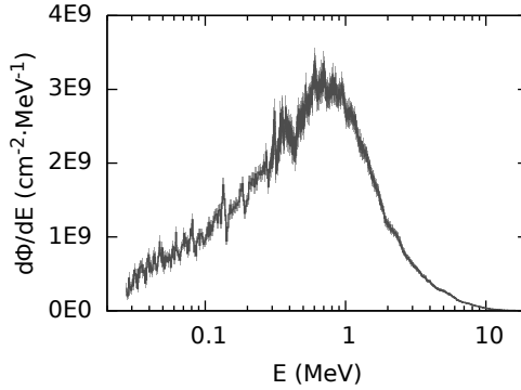
Figure 4.2: Neutron fluence energy distribution d\Phi/dE incident on the carbon sample as function of the neutron energy E (47.8 h measurement).
