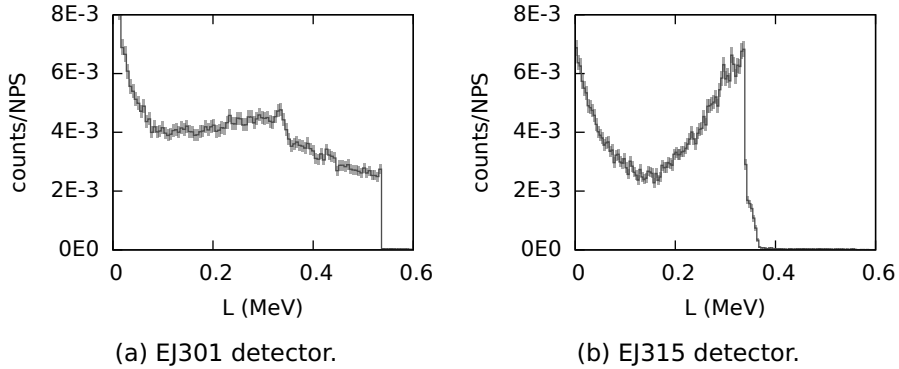
Figure 3.13: Light output spectra (counts per starting particle, NPS) simulated with MCNP for theoretical EJ301 and EJ315 detectors with infinitesimal resolution and for 2.0 MeV incident neutrons.
