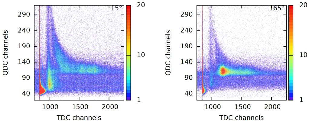
Figure 6.5: Example of raw data. The two-dimensional histograms show the counts as a function of the TDC time and QDC integrated charge recorded in almost 70 h of beam time, with the \text{CD}_2 sample as neutron scatterer, from one of the detectors at 15^\circ and one at 165^\circ .
