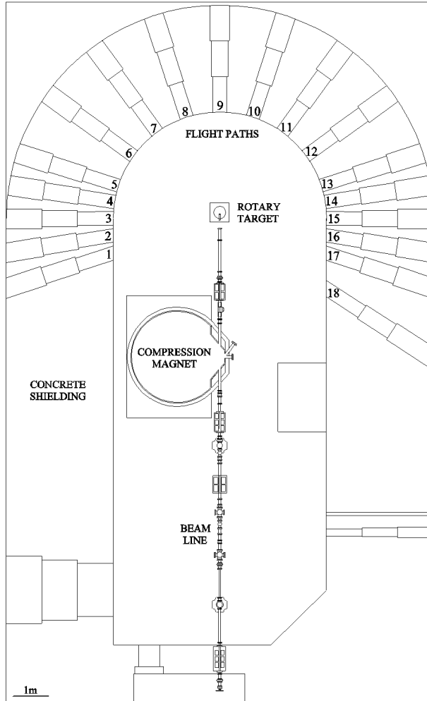
Figure 3.1: Scheme representing the main elements of GELINA: electron accelerator, compression magnet, uranium target, flight paths. Eighteen flight paths are in principle available, GELINA serves only twelve of them; flight paths 7, 8, 9, 10, 11 and 18 are not used. The present work made use of flight path 1, at 108^\circ to the electron beam.
