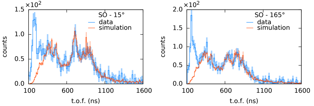
Figure 6.12: Experimental t.o.f. histograms (“data”) for the sample-out run, at 15^\circ and 165^\circ , compared to the simulated {}^6\text{Li}(n,\alpha) reaction rate tallied in the glass volume (“simulation”).
