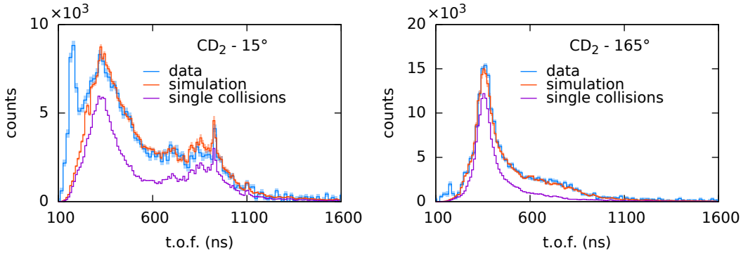
Figure 6.7: Experimental \text{CD}_2 t.o.f. histograms (“data”), at 15^\circ and 165^\circ , after the subtraction of the contribution of scattering in air, compared with the simulated {}^6\text{Li}(n,\alpha) reaction rate tallied in the detector sensitive volume (“simulation”). The “single collisions” lines are the simulation results when only neutrons arriving after a single collision on deuterium are considered.
