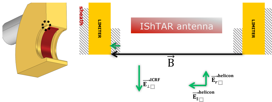
Figure 10: Schematic drawing of the antenna region where the electric field is measured. (a) The position with maximum electric field and (b) the geometry of the investigated region and configuration of RF and DC fields.
