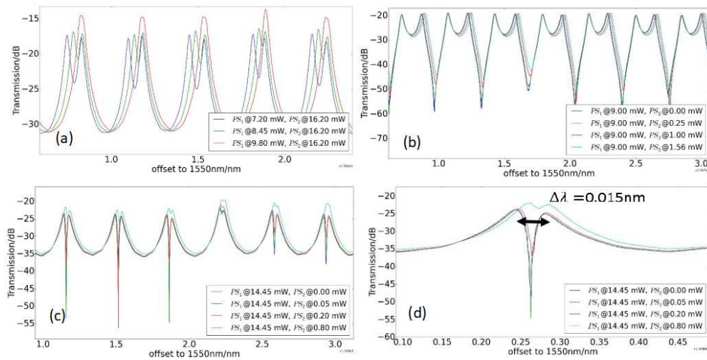
Fig. 7. Measured transmission spectra corresponding with the simulated spectra shown in Fig. 4. (a) presents the cases of Lorentzian-shaped resonance and normal resonance splitting where only one reflector introduces reflection. (b) indicates the Fano resonances when both reflectors introduce reflections. (c) gives the spectrum with EIT resonance. (d) provides a zoom view of one resonance in (c). It shows a bandwidth around 0.015 nm, or a Q factor around 1 \times 10^5 . All the measured spectra match well with simulations.
