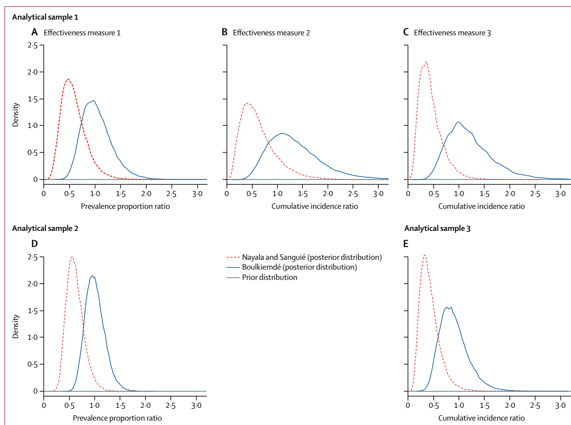
Figure 3: Prior and posterior distributions of the adjusted effect of the intervention in Boulkiemdé and in Nayala and Sanguié
