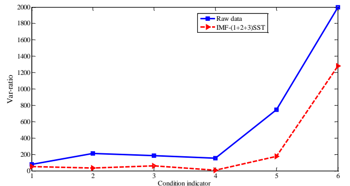
Figure 9: Uncertainties in the condition indicator estimates
