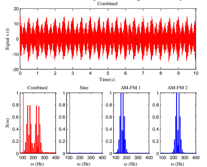
Figure 1: Signal and its components
