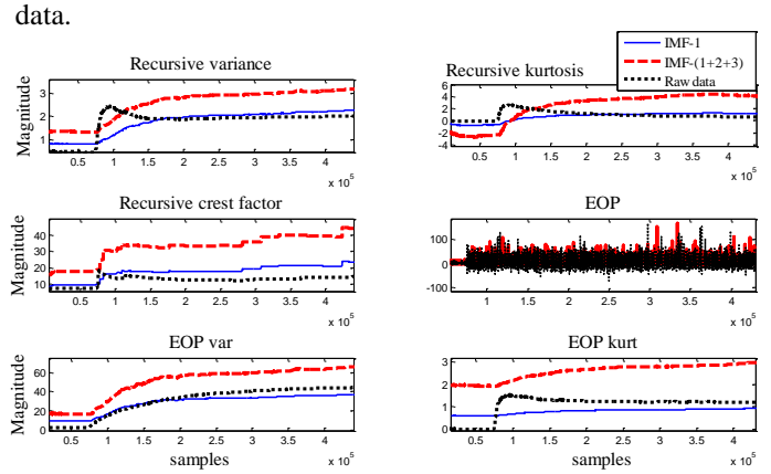
Figure 8: Recursive condition indicators applied on the raw data and IMFs
