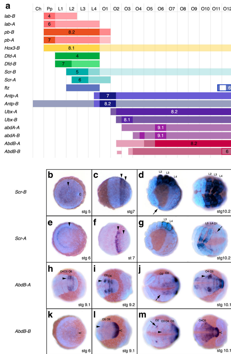
Fig. 9 Expression of Hox paralogs in P. tepidarium . a Summary of Hox gene expression domains and expression timing in P. tepidarium embryos. Columns represent segments from anterior to posterior. Bars represent the extent of a gene's expression domain with respect to the segments. The darkest color for each gene is used for the initial expression domain of each gene when it first appears, which usually coincides with a gene's strongest expression. The next lighter color is used for the expanded domain, and the lightest color is used for further late expansions of the expression domains, which usually tends to be only in the nervous system. The stage at which a gene's expression first appears is depicted by the stage number in the domain of first expression. ftz , in addition to its Hox domain, is expressed dynamically (i.e., budding off stripes) in the SAZ, and AbdB-B is continuously expressed in the SAZ after its formation at stage 6. These SAZ expression patterns are indicated by rectangular outlines in what is otherwise the O12 segment. Note that, since we did not detect clear expression boundaries for Hox3-A , the expression of this gene is not represented. b–m Two examples of Hox gene expression differences between paralogs of Scr ( b–g ) and AbdB ( h–m ). For detailed descriptions of expression patterns, see Additional file 44: Supplementary File 1 and the legends of Additional file 33: Figure S17, Additional file 34: Figure S18, Additional file 42: Figure S26, Additional file 43: Figure S27. All images are overlays of a bright-field images depicting the expression pattern and a fluorescent DAPI nuclear staining. Abbreviations: Ch cheliceral segment, Pp Pedipalpal segment, L–L4 walking leg segments 1–4, O1–12 opisthosomal segments 1–12
