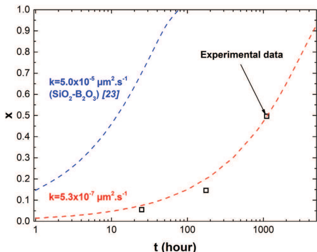
Fig. 9. Evolution of the oxidation ratio ( x ) of spherical \text{MoSi}_2 based particles as a function of time at a temperature of 1100\text{ }^\circ\text{C} .
