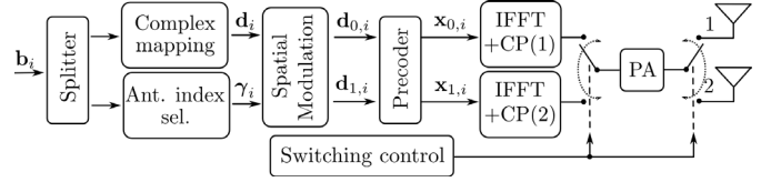
Fig. 1. Block diagram of the transmitter.
