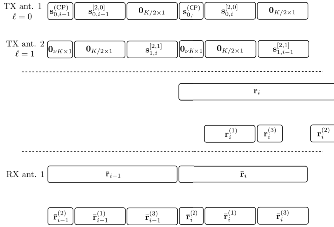
Fig. 3. Time domain representations of some of the vectors described in the proposed processing that appear during time slots i - 1 and i -th.
