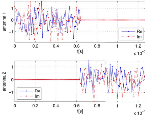
Fig. 2. Time domain signals in each of the two available antenna ( N_T = 2 ) for a configuration with bandwidth of 10 MHz and 128 subcarriers.
