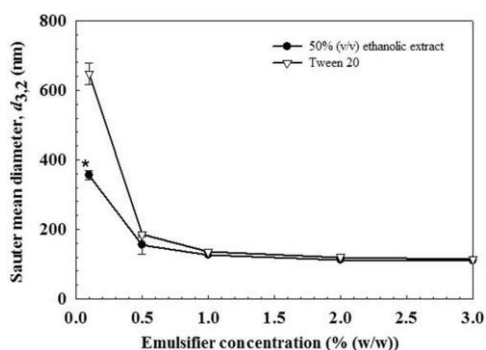
Fig. 3 Effect of emulsifier concentration on the Sauter mean diameter ( d_{3,2} ) of 10% (w/w) soybean O/W emulsions prepared using a high-pressure homogenizer (100 MPa, 4 passes). *A small layer of oil was observed on the top of this sample.
