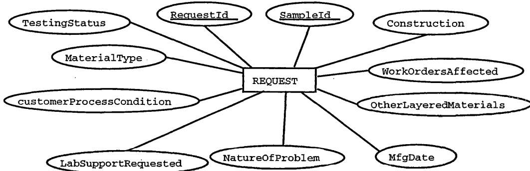
Figure 7c. Request Entity Properties
