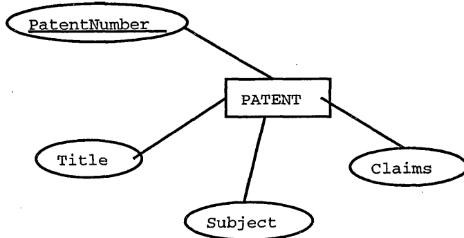
Figure 8b. Patent Entity Properties
