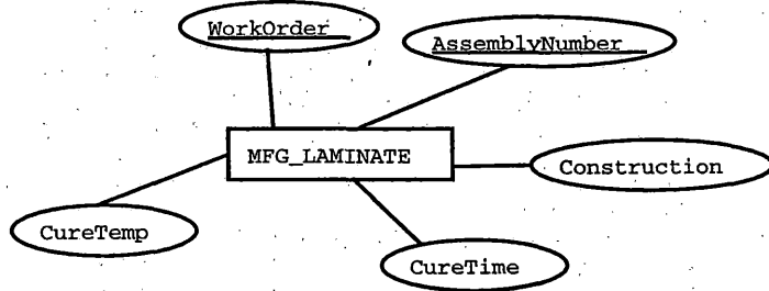
Figure 5c. Manufacturing Laminate Entity Properties
