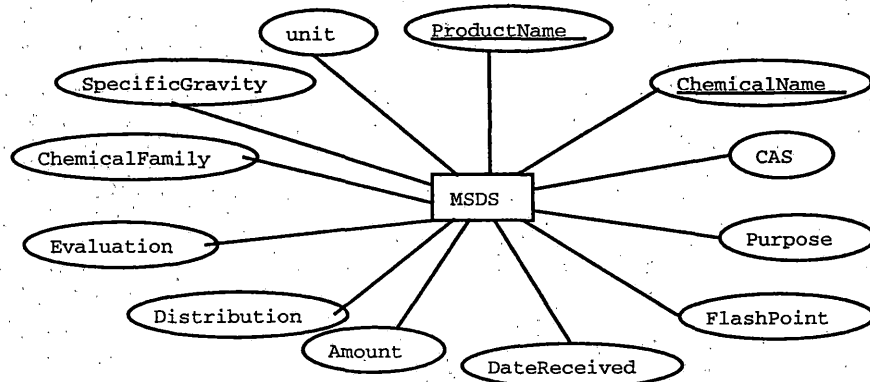
Figure 5b. Manufacturing DataSheet Entity Properties
