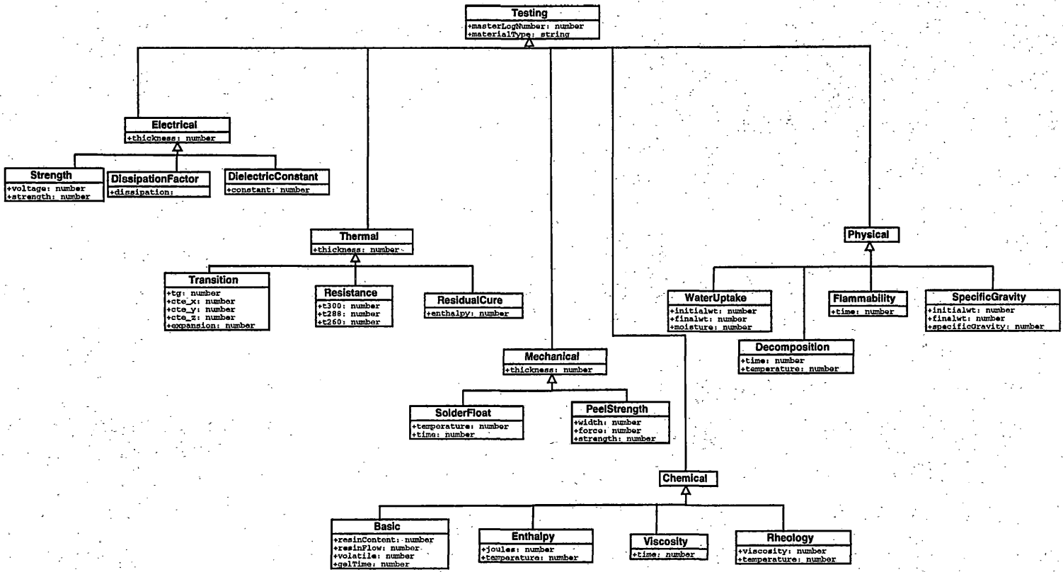
Figure 10. Object-Oriented Model: Technical Service Support
