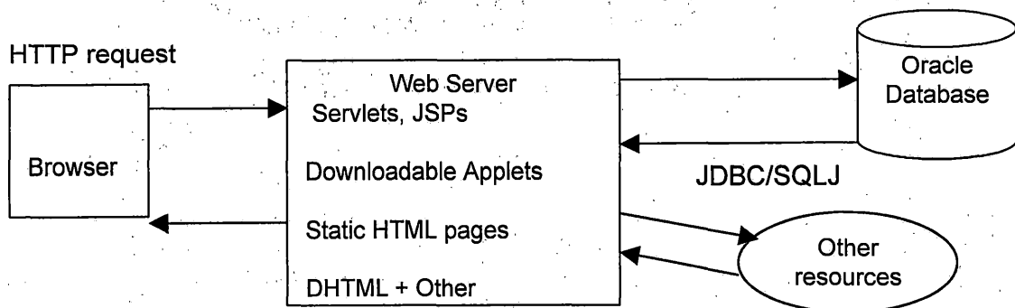
Figure 1. General Overview of the Interactive System
