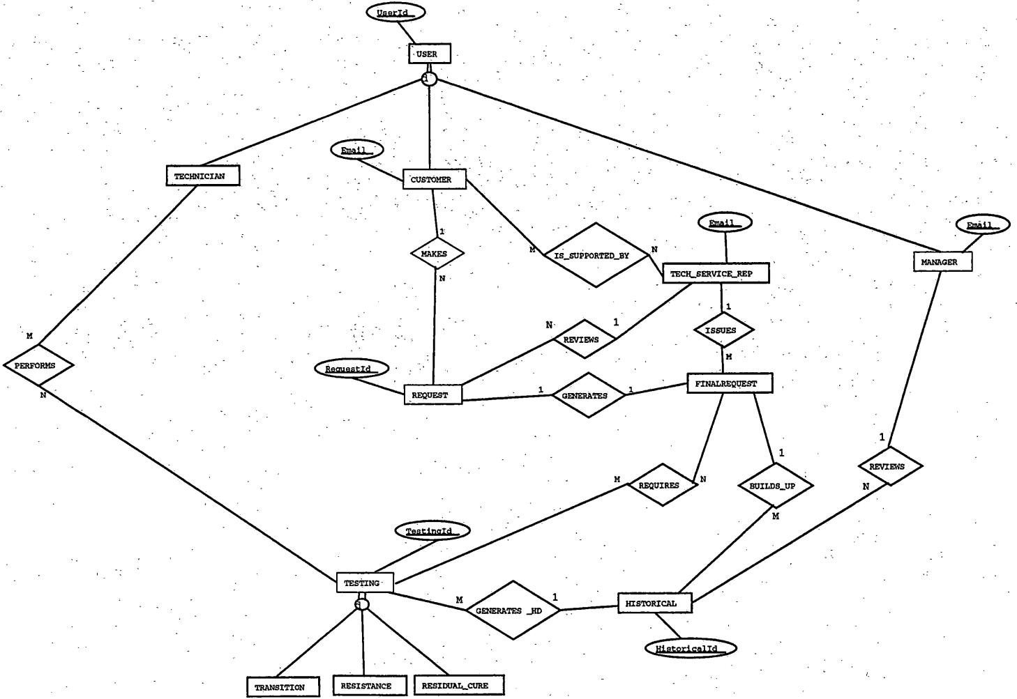
Figure 3. Entity Enhanced Relational Diagram: Technical Service Support
