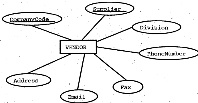
Figure 5a. Vendor Entity Properties
