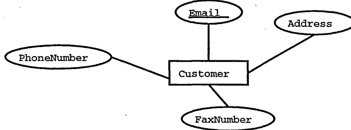
Figure 7b. Customer Entity Properties
