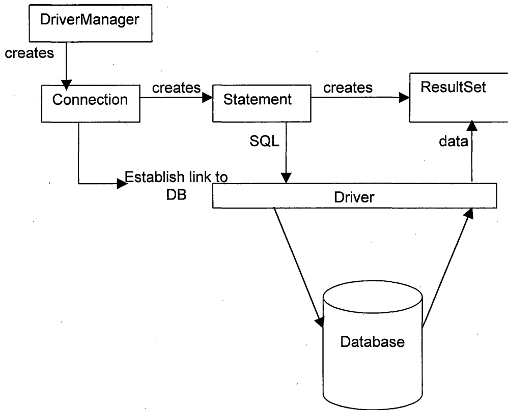
Figure 12. Java Database Connectivity Architecture
