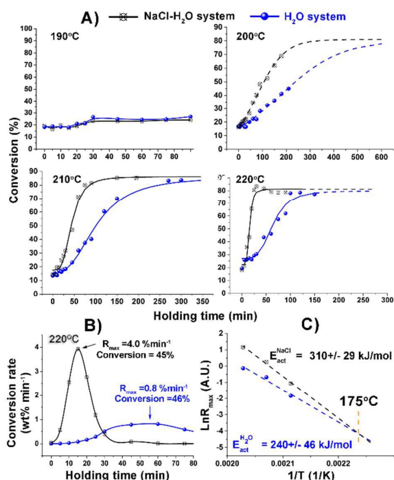
Fig. 1 (A) Cellulose conversion in \text{H}_2\text{O} and \text{NaCl-H}_2\text{O} systems at different reaction temperatures; (B) conversion rate of cellulose in \text{H}_2\text{O} and \text{NaCl-H}_2\text{O} systems at 220^\circ\text{C} ; (C) total activation energy.
