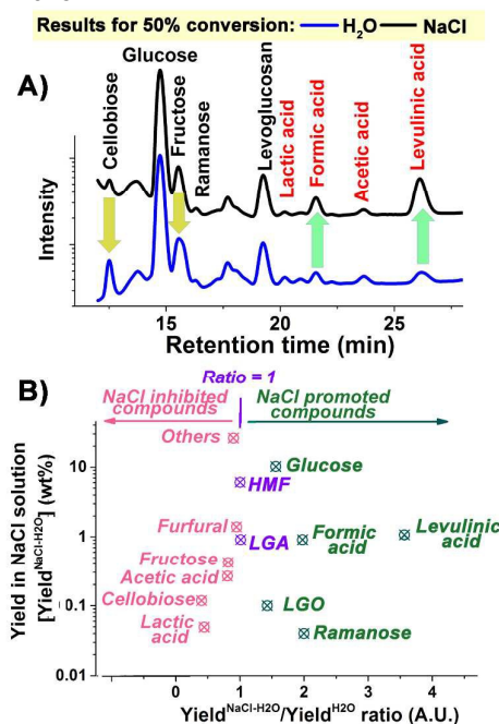
Fig. 2 (A) HPLC signal traces and (B) \text{NaCl} effect of the products formed at 50% conversion of cellulose in \text{H}_2\text{O} and \text{NaCl-H}_2\text{O} systems at 210^\circ\text{C} .
