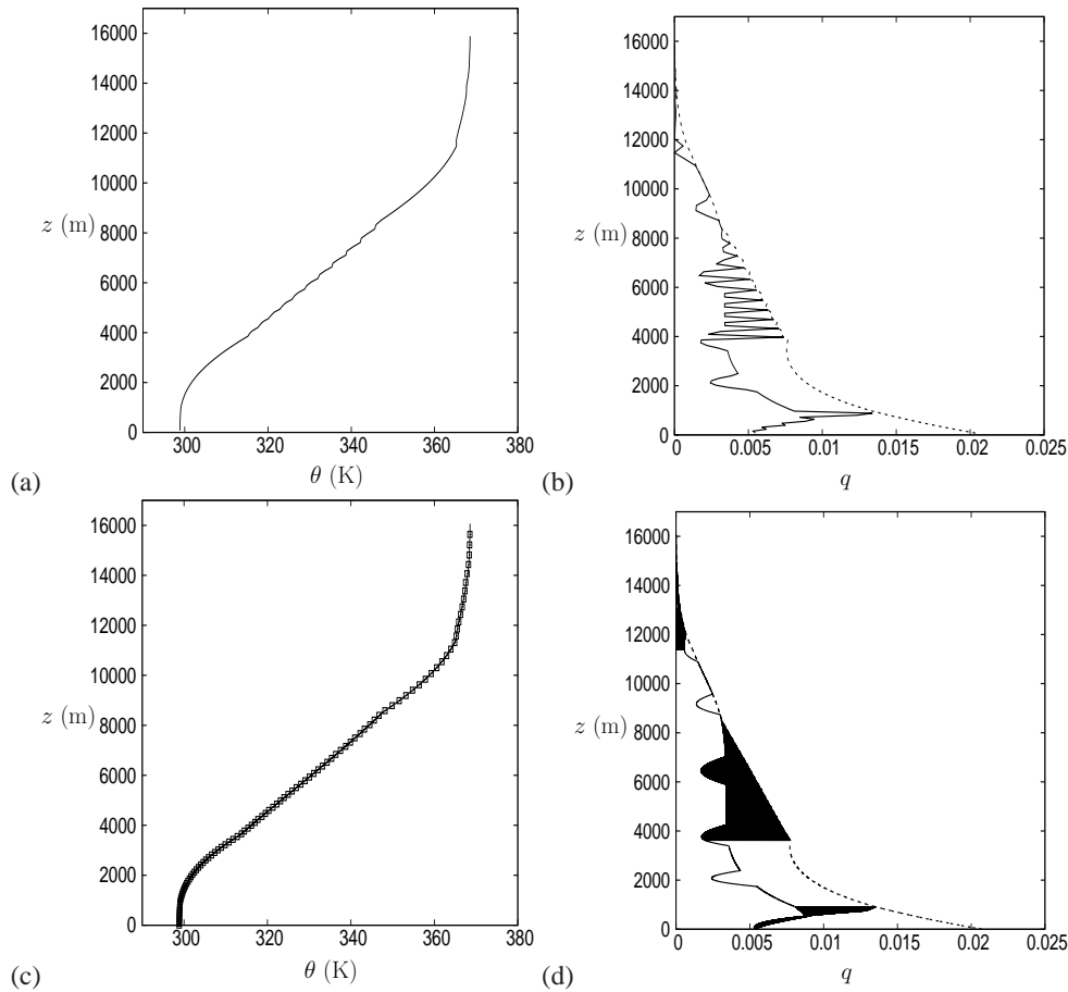
Figure 6. Plot of (a,c) the final potential temperature distribution \theta(z) and (b,d) the final moisture distribution q(z) after the moist convective adjustment for the initial data given in figure 5. In panels (a,b) N = 100 and (c,d) N = 10000 . The dashed lines give the value of Q_{\text{sat}} after the rearrangement. In panel (c) the squares correspond to the solution minimising F_{\infty}[K] with N = 2000 parcels. Only every 20 parcels are plotted for clarity.
