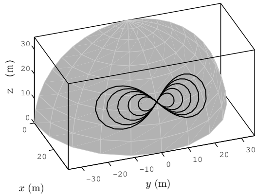
Fig. 15. Reference path for different values of u_2 = \{-0.2, -0.1, 0, 0.1, 0.2\} , with u_1 = 0 .
