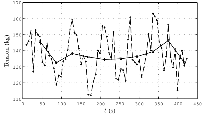
Fig. 19. No averaging (dashed with crosses), averaging over N_{\text{avg}} = 7 path cycles (solid with circles). During this experiment, the kite followed a constant reference path.
