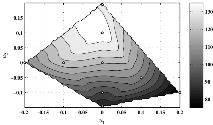
Fig. 22. Contour plot of the average line tension in kg (shading) per figure-of-eight vs. \mathbf{u} . At each of the data points (circles), the average line tension during 10 minutes of experimental data was recorded. The surface was estimated by performing a piecewise-cubic interpolation of these data points.
