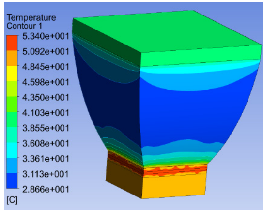
FIGURE 3. ANSYS simulation of CCPC optics showing a maximum temperature of 53°C at the cell surface
